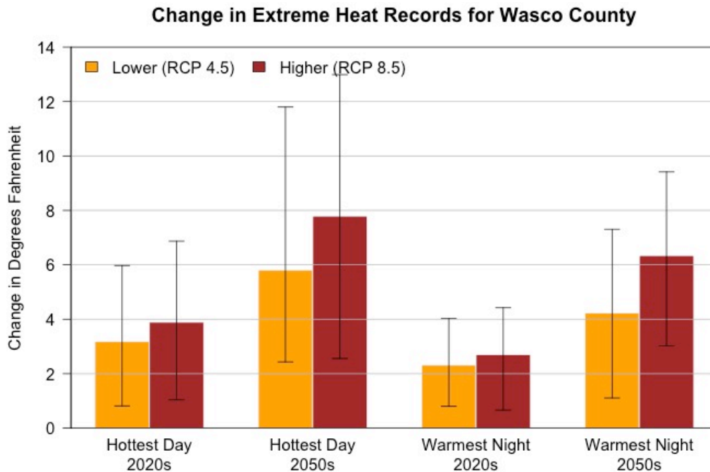
Figure 5 Projected future changes in the hottest day of the year (left two sets of bars) and warmest night of the year (right two sets of bars) for Wasco County from the historical baseline (1971–2000 average) for the 2020s (2010–2039 average) and 2050s (2040–2069 average) under a lower (RCP 4.5) and higher (RCP 8.5) emissions scenario based on 20 global climate models. The bars and whiskers display the mean and range, respectively, of changes across the 20 GCMs.
