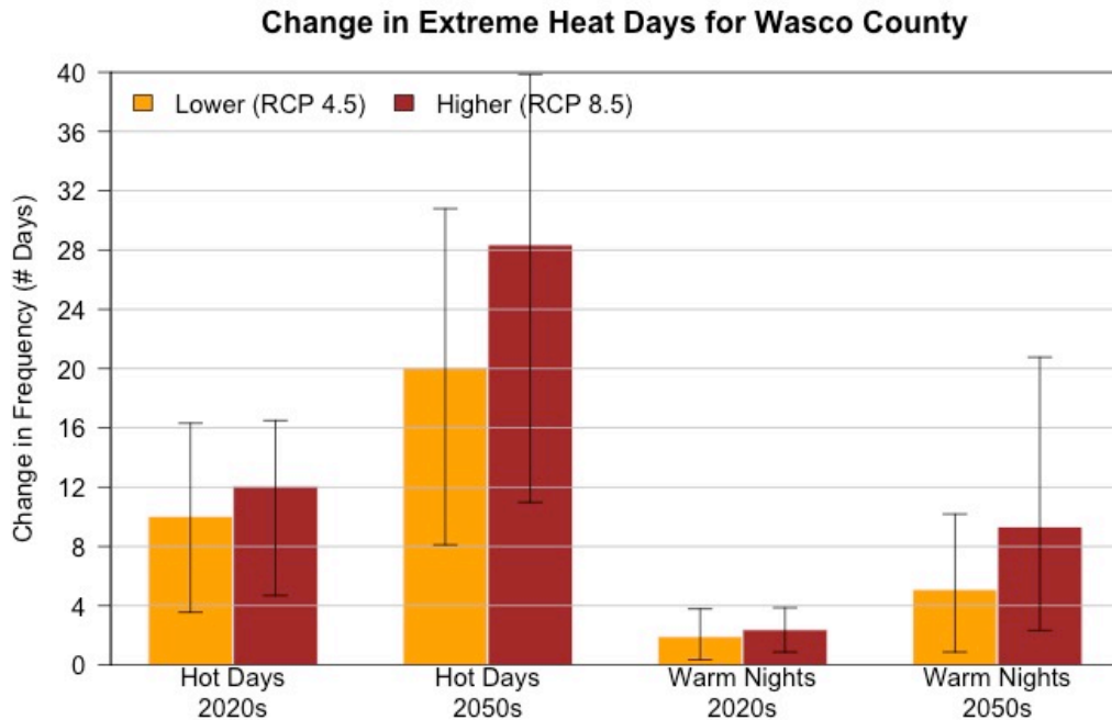
Figure 4 Projected future changes in the number of hot days (left two sets of bars) and number of warm nights (right two sets of bars) for Wasco County from the historical baseline (1971–2000 average) for the 2020s (2010–2039 average) and 2050s (2040–2069 average) under a lower (RCP 4.5) and higher (RCP 8.5) emissions scenario based on 20 global climate models. The bars and whiskers display the mean and range, respectively, of changes across the 20 GCMs. Hot days are defined as days with maximum temperature of at least 90°F; warm nights are defined as days with minimum temperature of at least 65°F.
