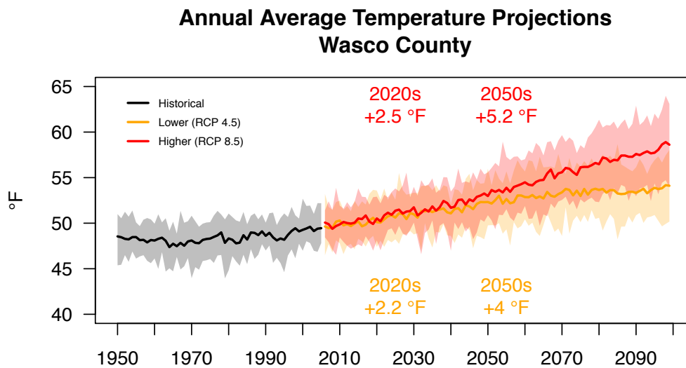
Figure 3 Annual average temperature projections for Wasco County as simulated by 20 downscaled global climate models under a lower (RCP 4.5) and a higher (RCP 8.5) greenhouse gas emissions scenario. Solid line and shading depicts the 20-model mean and range, respectively. The multi-model mean differences for the 2020s (2010–2039 average) and the 2050s (2040–2069 average) compared to the historical baseline (1971–2000 average) are shown.
