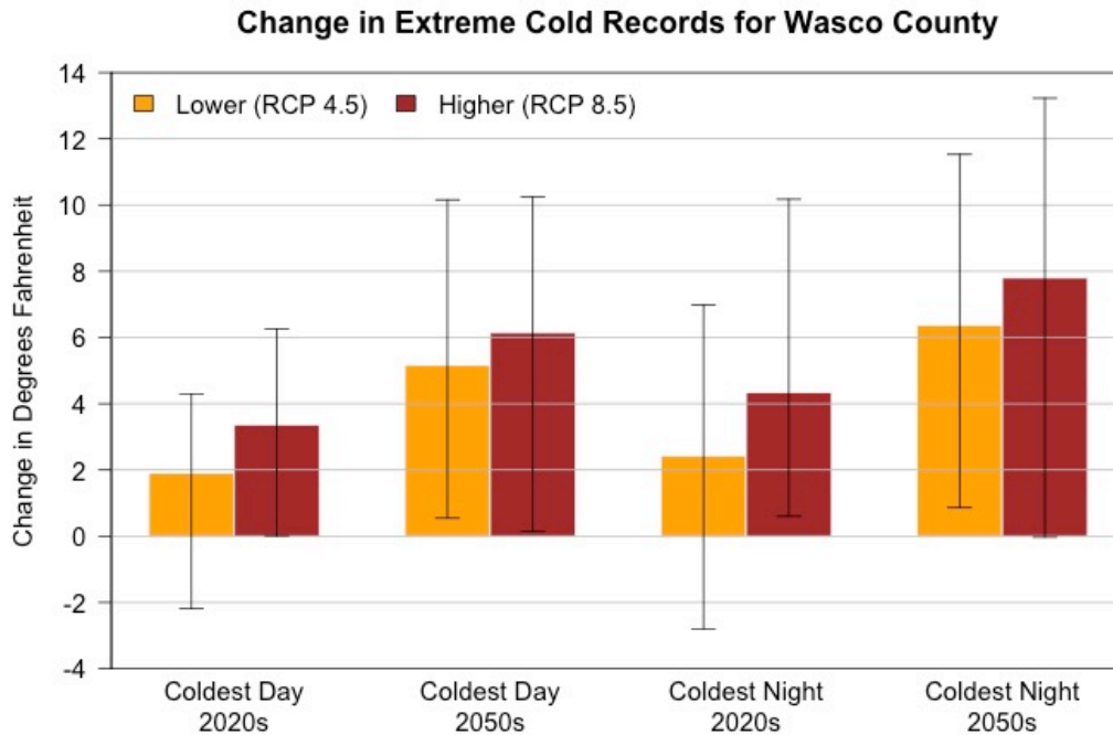
Figure 8 Projected future changes in the coldest day of the year (left two sets of bars) and coldest night of the year (right two sets of bars) for Wasco County from the historical baseline (1971–2000 average) for the 2020s (2010–2039 average) and 2050s (2040–2069 average) under a lower (RCP 4.5) and higher (RCP 8.5) emissions scenario based on 20 global climate models. The bars and whiskers display the mean and range, respectively, of changes across the 20 GCMs.
