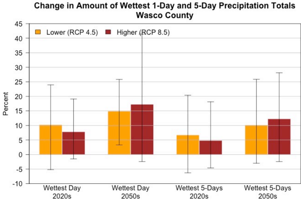
Figure 10 Projected future changes in the wettest day of the year (left two sets of bars) and wettest consecutive five days of the year (right two sets of bars) for Wasco County from the historical baseline (1971–2000 average) for the 2020s (2010–2039 average) and 2050s (2040–2069 average) under a lower (RCP 4.5) and higher (RCP 8.5) emissions scenario based on 20 global climate models. The bars and whiskers display the mean and range, respectively, of changes across the 20 GCMs.
