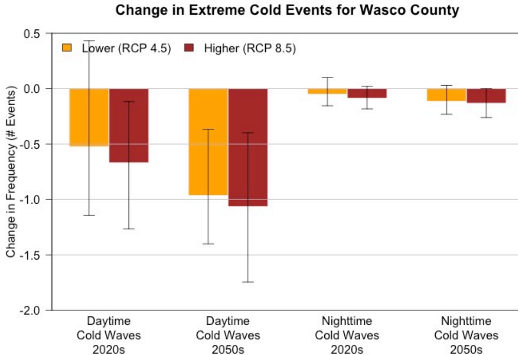
Figure 9 Projected future changes in the number of daytime cold waves (left two sets of bars) and number of nighttime cold waves (right two sets of bars) for Wasco County from the historical baseline (1971–2000 average) for the 2020s (2010–2039 average) and 2050s (2040–2069 average) under a lower (RCP 4.5) and higher (RCP 8.5) emissions scenario based on 20 global climate models. The bars and whiskers display the mean and range, respectively, of changes across the 20 GCMs. Daytime cold waves are defined as events with three or more consecutive days with maximum temperature at or below 32°F; nighttime cold waves are defined as events with three or more consecutive days with minimum temperature at or below 0°F.
