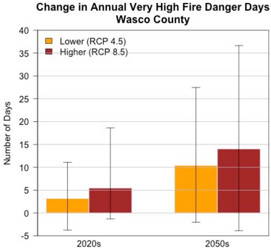
Figure 15 Projected future changes in the frequency of very high fire danger days for Wasco County from the historical baseline (1971–2000 average) for the 2020s (2010–2039 average) and 2050s (2040–2069 average) under a lower (RCP 4.5) and higher (RCP 8.5) emissions scenario based on 18 global climate models. The bars and whiskers display the mean and range, respectively, of changes across the 18 GCMs. (Data Source: Northwest Climate Toolbox, climatetoolbox.org/tool/Climate-Mapper )
