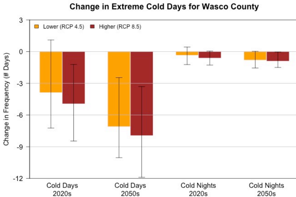
Figure 7 Projected future changes in the number of cold days (left two sets of bars) and number of cold nights (right two sets of bars) for Wasco County from the historical baseline (1971–2000 average) for the 2020s (2010–2039 average) and 2050s (2040–2069 average) under a lower (RCP 4.5) and higher (RCP 8.5) emissions scenario based on 20 global climate models. The bars and whiskers display the mean and range, respectively, of changes across the 20 GCMs. Cold days are defined as days with maximum temperature at or below 32°F; cold nights are defined as days with minimum temperature at or below 0°F.
