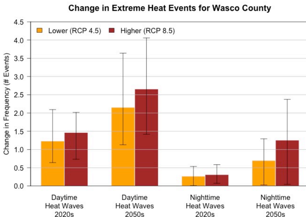
Figure 6 Projected future changes in the number of daytime heat waves (left two sets of bars) and number of nighttime heat waves (right two sets of bars) for Wasco County from the historical baseline (1971–2000 average) for the 2020s (2010–2039 average) and 2050s (2040–2069 average) under a lower (RCP 4.5) and higher (RCP 8.5) emissions scenario based on 20 global climate models. The bars and whiskers display the mean and range, respectively, of changes across the 20 GCMs. Daytime heat waves are defined as events with three or more consecutive days with maximum temperature of at least 90°F; nighttime heat waves are defined as events with three or more consecutive days with minimum temperature of at least 65°F.
