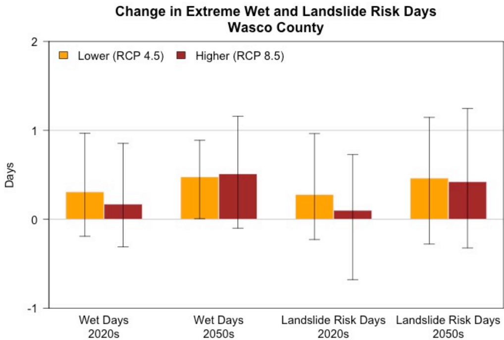
Figure 11 Projected future changes in the frequency of wet days (left two sets of bars) and landslide risk days (right two sets of bars) for Wasco County from the historical baseline (1971–2000 average) for the 2020s (2010–2039 average) and 2050s (2040–2069 average) under a lower (RCP 4.5) and higher (RCP 8.5) emissions scenario based on 20 global climate models. The bars and whiskers display the mean and range, respectively, of changes across the 20 GCMs.
