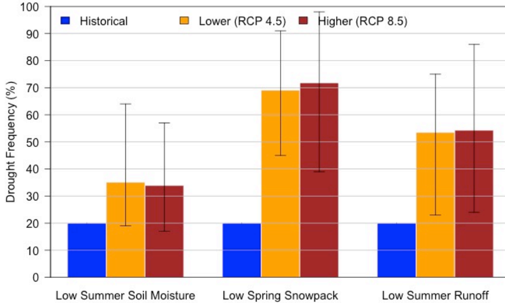
Figure 14 Frequency of the historical baseline (1971–2000) 1-in-5 year event (by definition 20% frequency) of low summer soil moisture (average of June–July–August), low spring snowpack (April 1 snow water equivalent), and low summer runoff (average of June–July–August) for the future period 2040–2069 for lower (RCP 4.5) and higher (RCP 8.5) emissions scenarios. The bar and whiskers depict the mean and range across ten global climate models. (Data Source: Integrated Scenarios of the Future Northwest Environment, https://climate.northwestknowledge.net/IntegratedScenarios/ )
