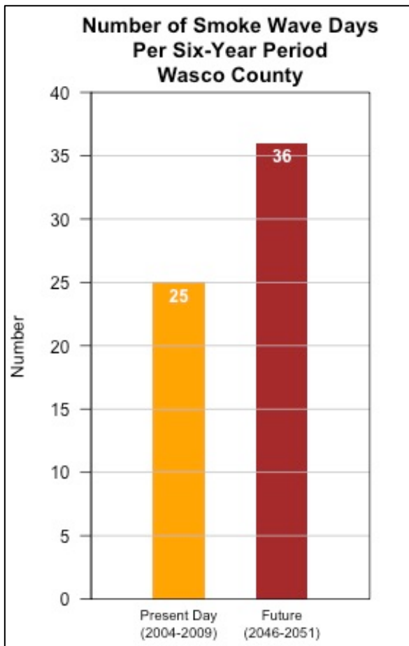
Figure 16 Simulated present day (2004–2009) and future (2046–2051) frequency of “smoke wave” days for Wasco County under a medium emissions scenario 11 . The bars display the mean across 15 GCMs. (Data source: Liu et al. 2016, https://khanotations.github.io/smoke-map/ )
