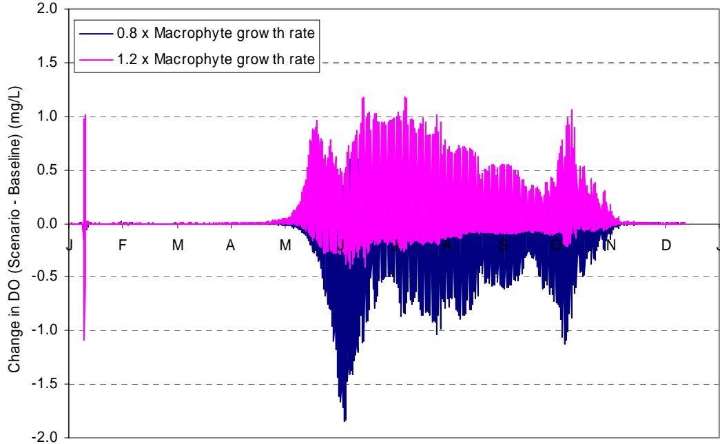
F_1999-8 Macrophyte growth rate sensitivity simulation - Lost River at Keller Bridge (LRKB)
