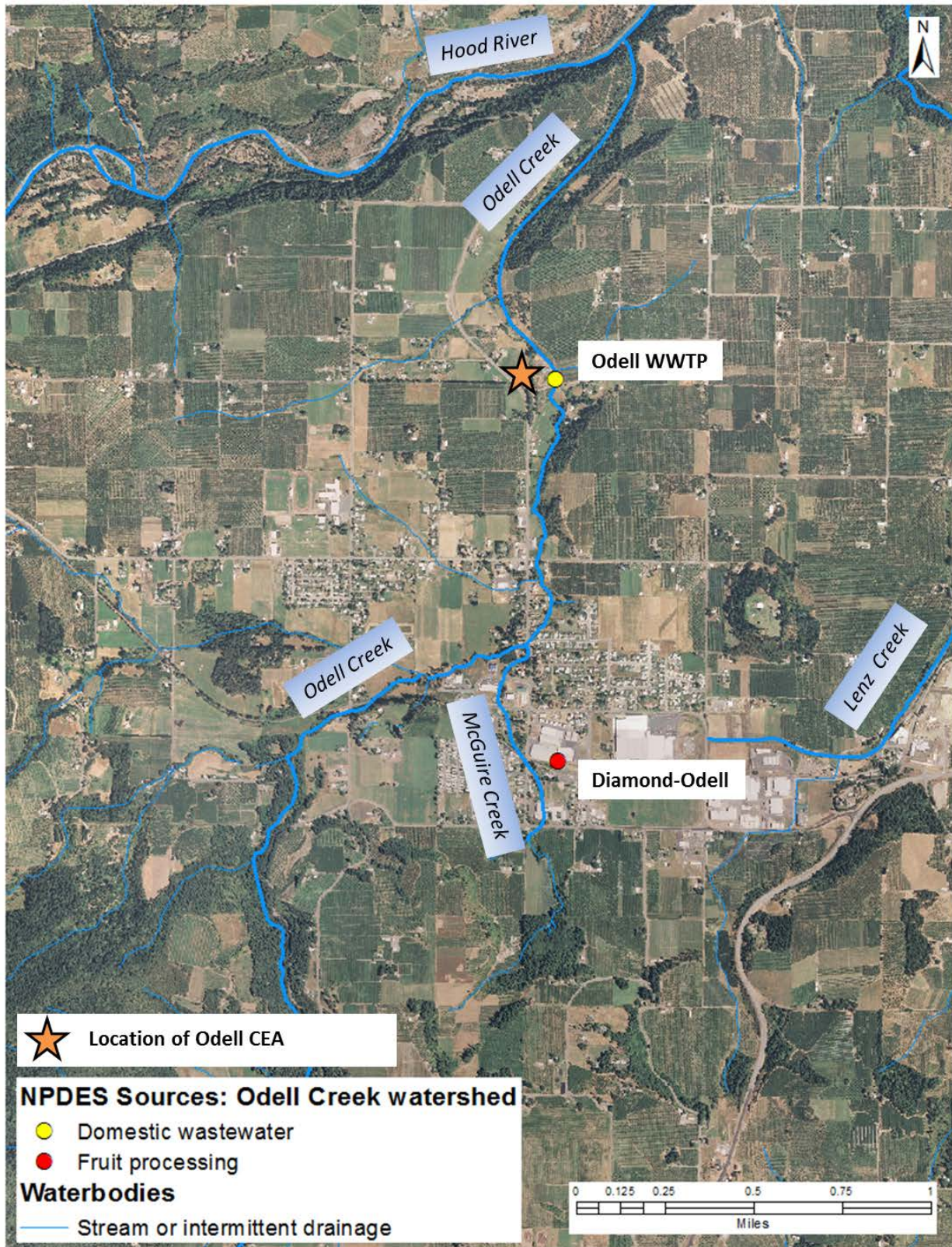
Figure B-2. Location of NPDES facilities within the Odell Creek watershed
