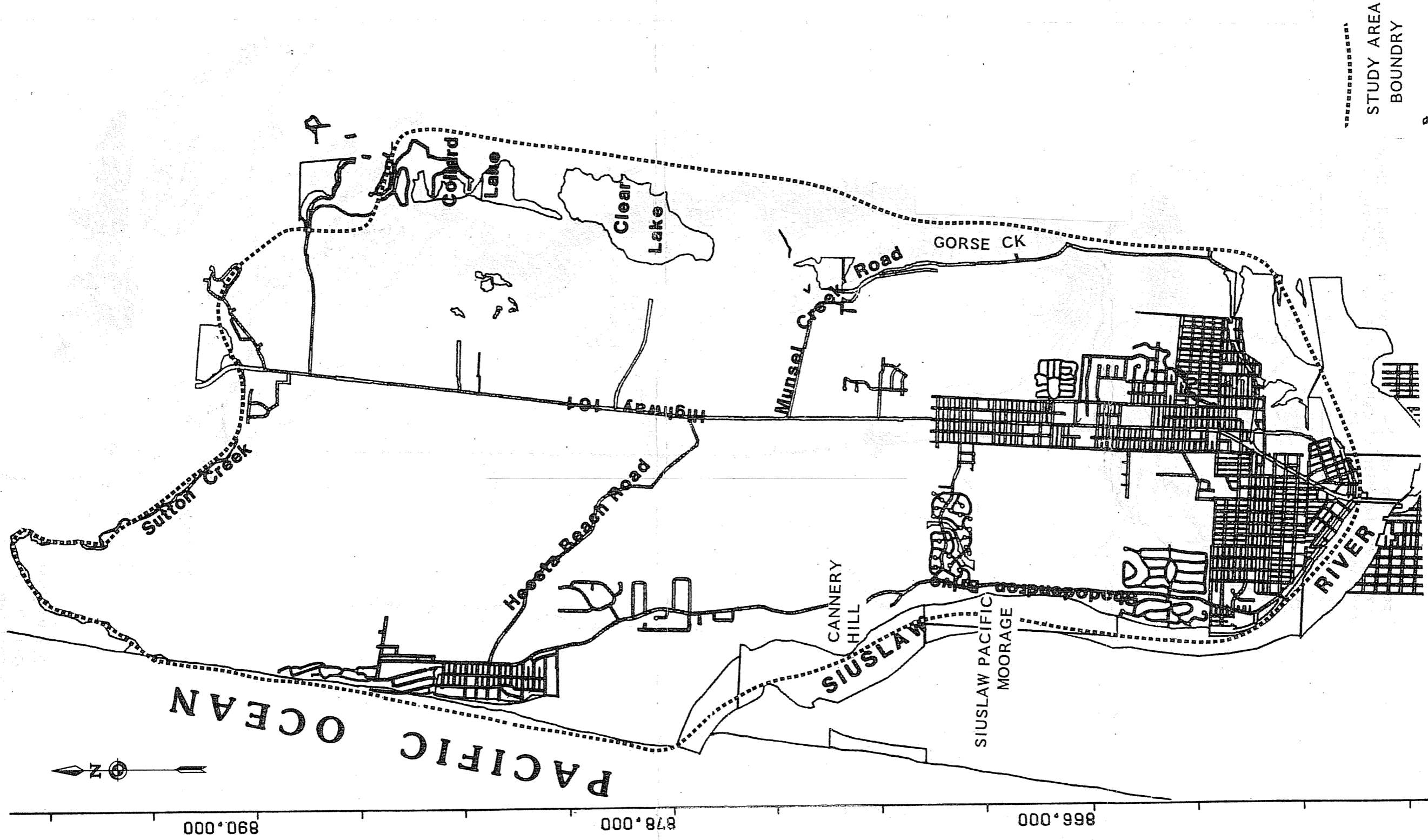
FIGURE 2. Locator Map for the North Florence Dunal Aquifer Showing Study Area Boundaries, Roads, Streams and Lakes.
