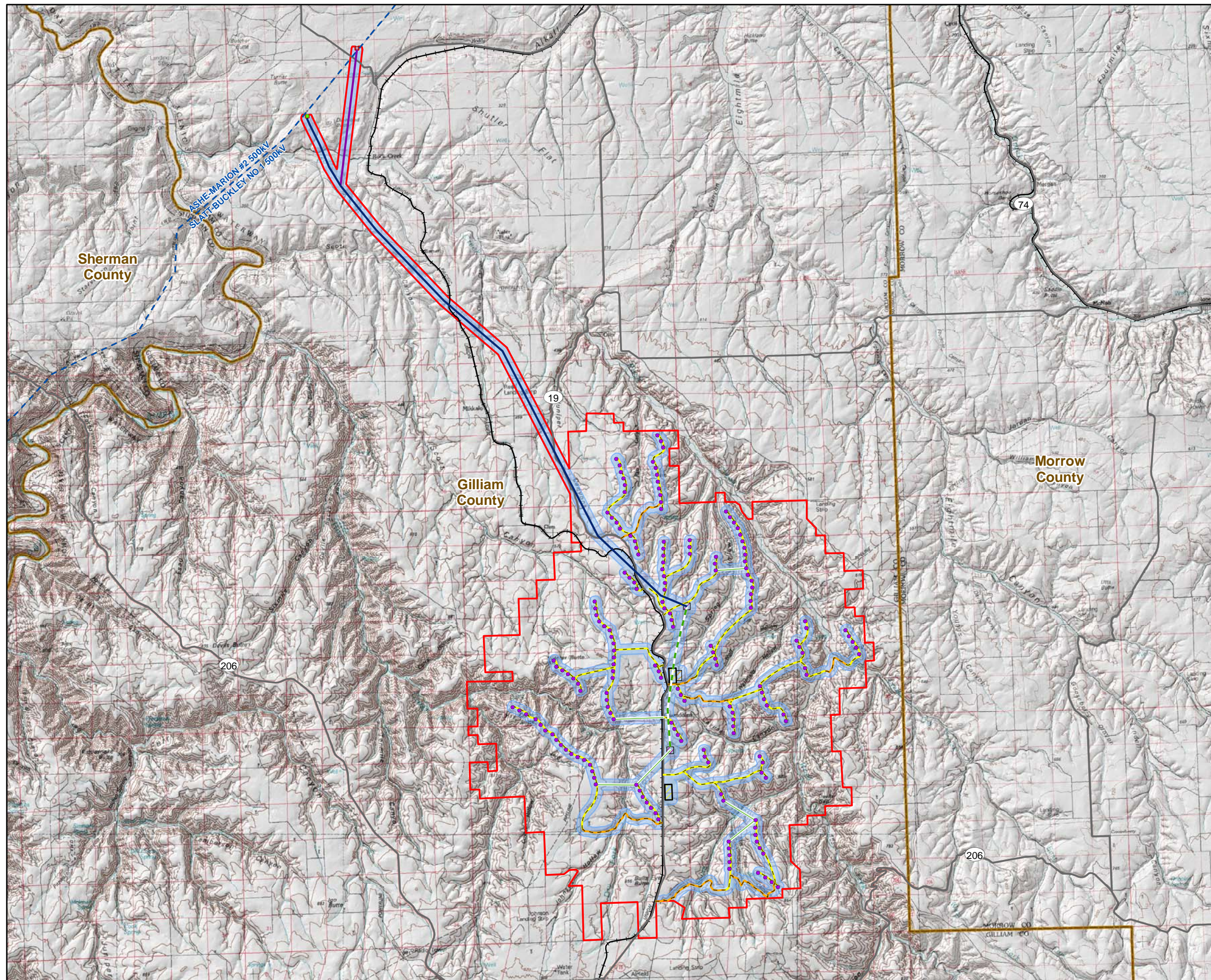
FIGURE G-2 Facility Layout Rock Creek Wind Power Facility Notice of Intent
