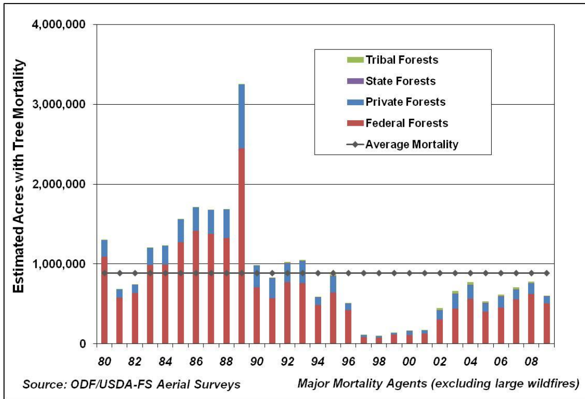
Figure 1: Estimated annual area (acres) containing tree mortality and the long-term average for Oregon forest lands as assessed by aerial surveys (1980-2009). 1, 2
