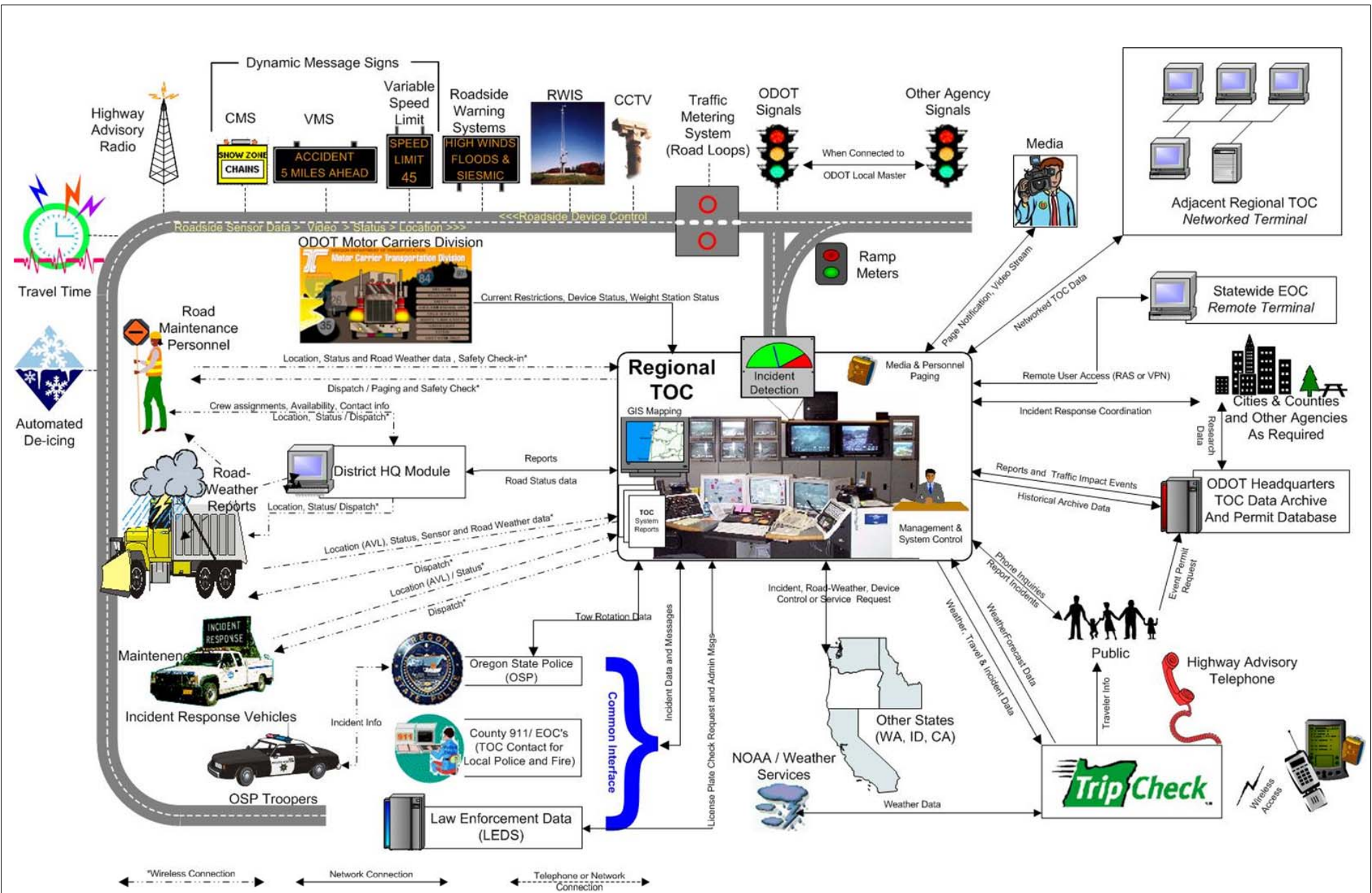
Figure 9 ODOT REGIONAL TOC CONCEPT OF OPERATIONS
