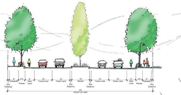
ESTACADA - OR 224 Streetscape Section A/A Cross Section - Typical not to scale
