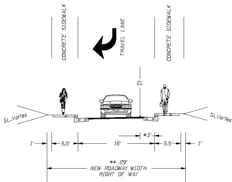
South 32nd Street Jug Handle Turnaround
