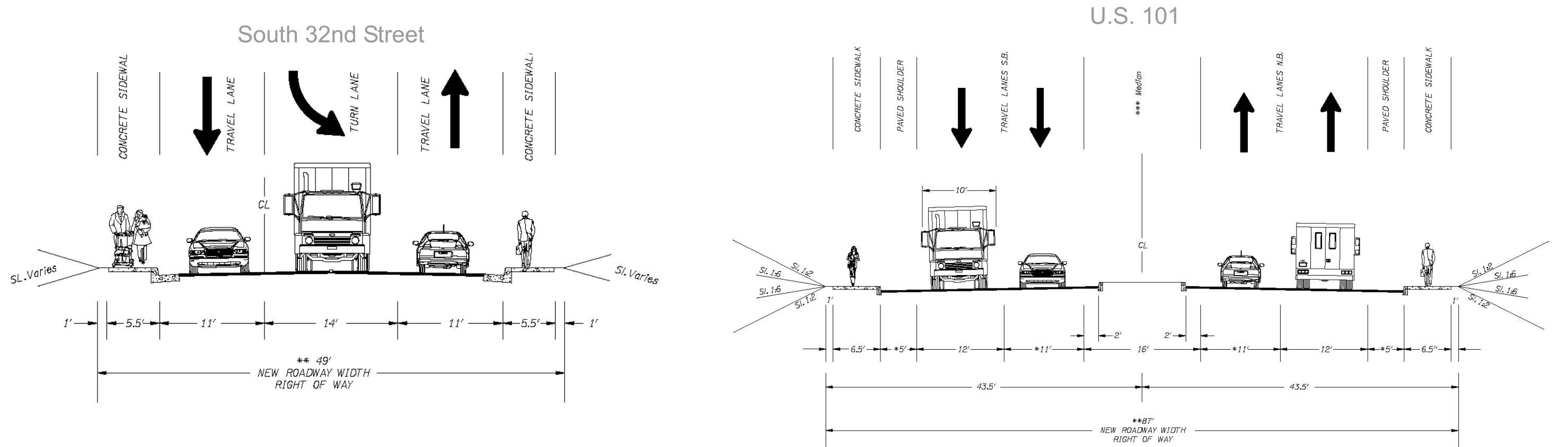
South 32nd Street Jug Handle Turnaround
