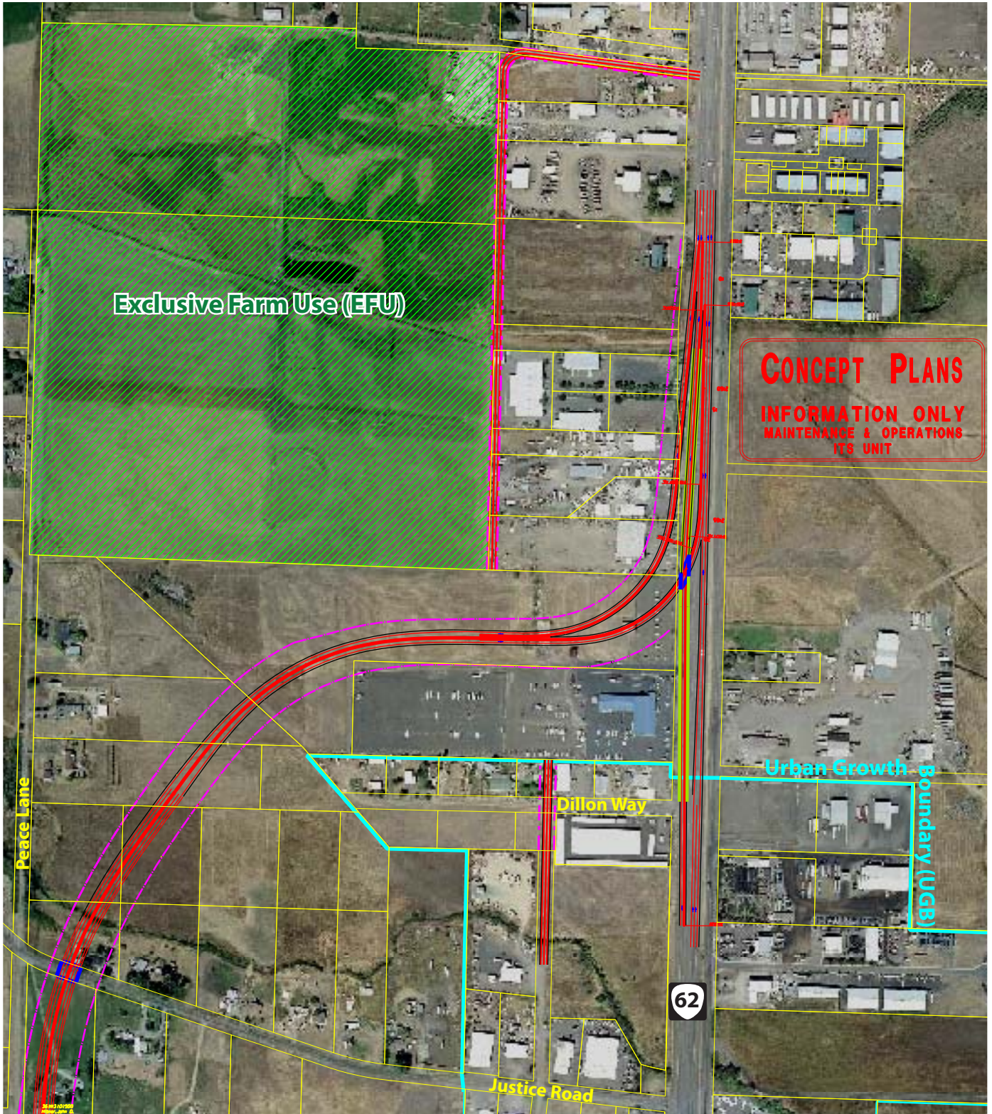
North Terminus: Free-Flow Interchange Option
