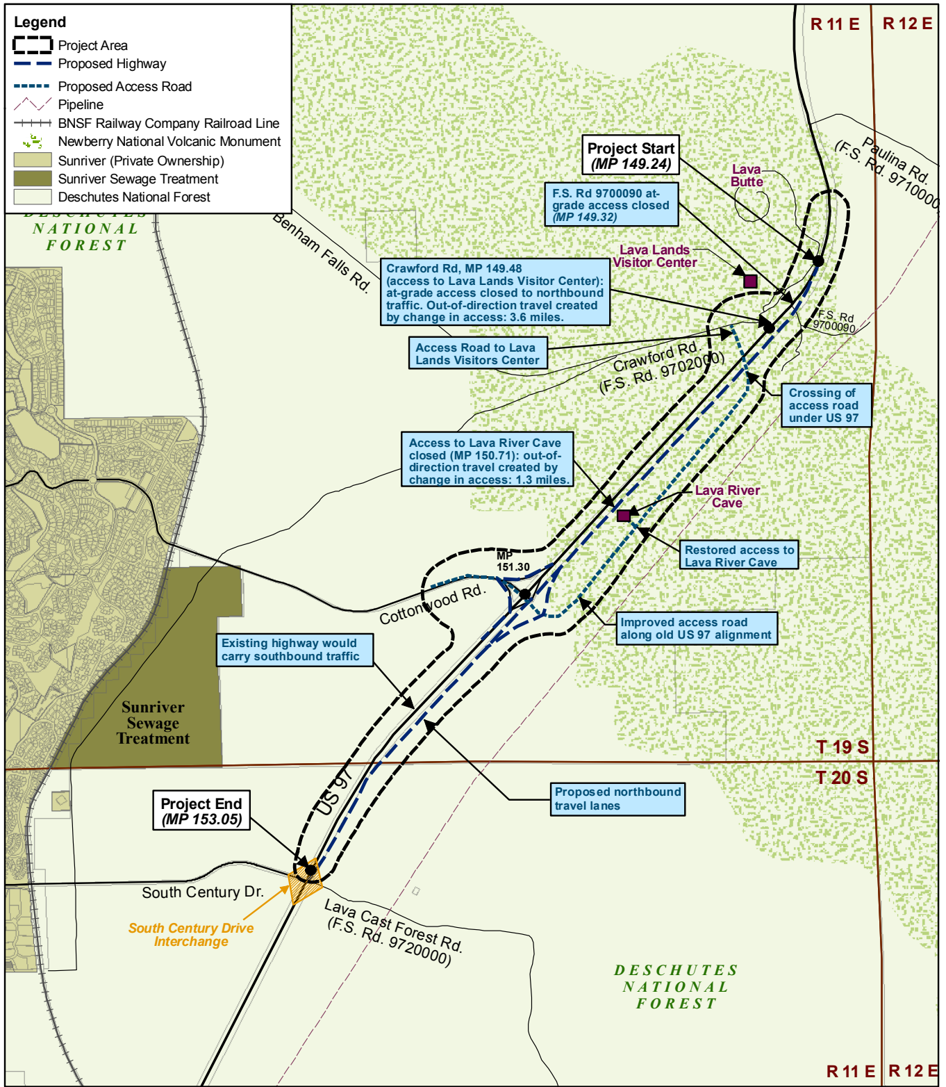
Figure 2 Build Alternative
