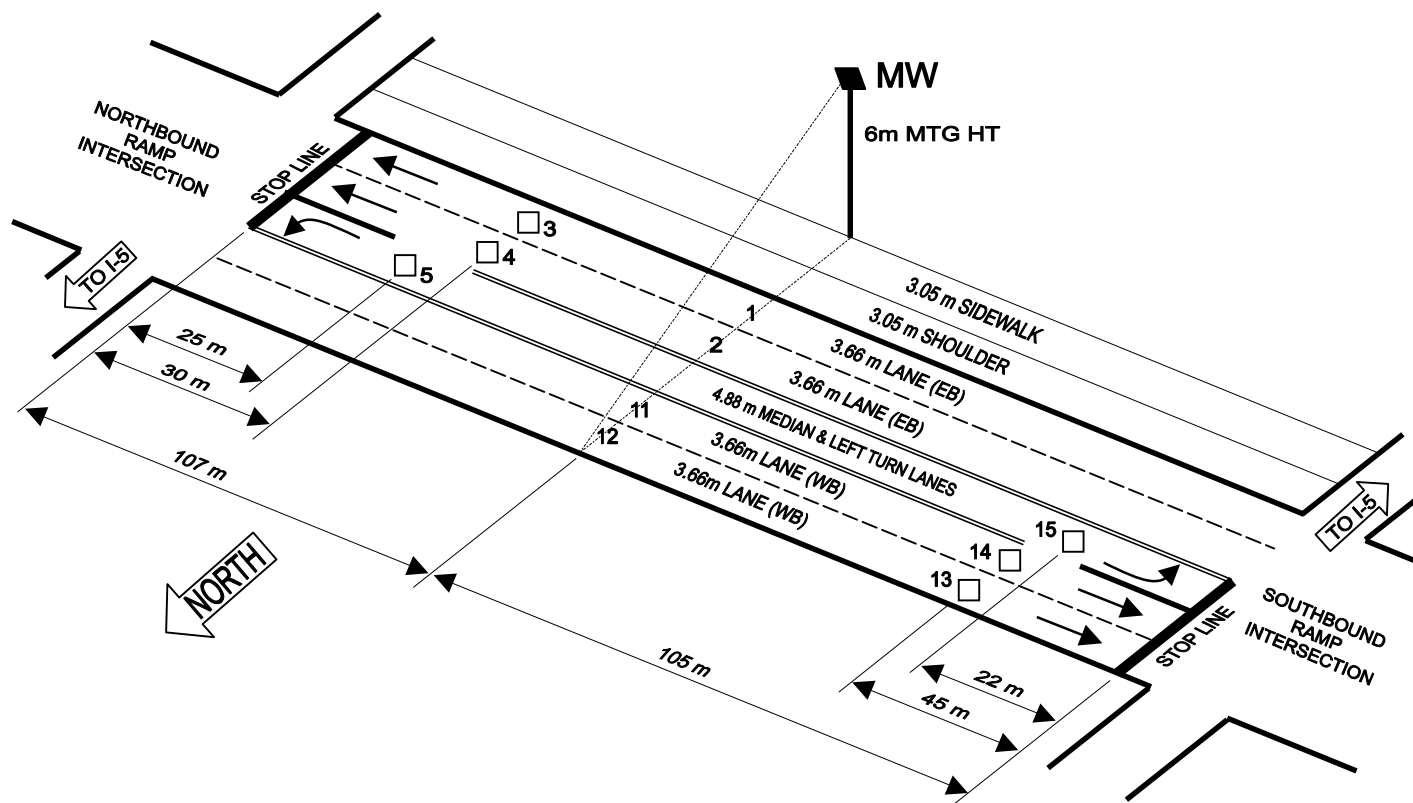
Figure 1.1 Layout of Microwave and Loop Sensors on Chemawa Road
