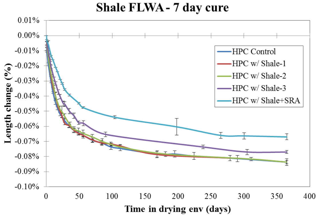
Figure 5.12: Drying shrinkage results, 7 day cure (shale FLWA mixtures)
