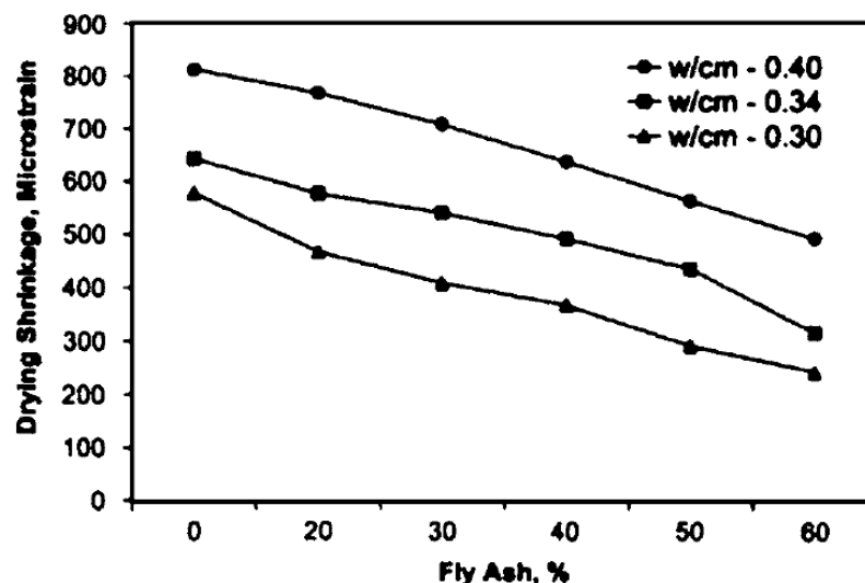
Figure 2.2: Variation of drying shrinkage of concrete with varying fly ash content (Kumar et al. 2007)
