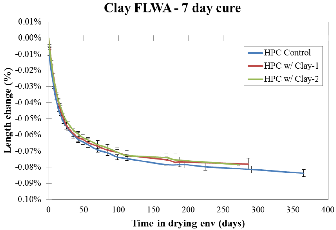
Figure 5.9: Drying shrinkage results, 7 day cure (clay FLWA mixtures)
