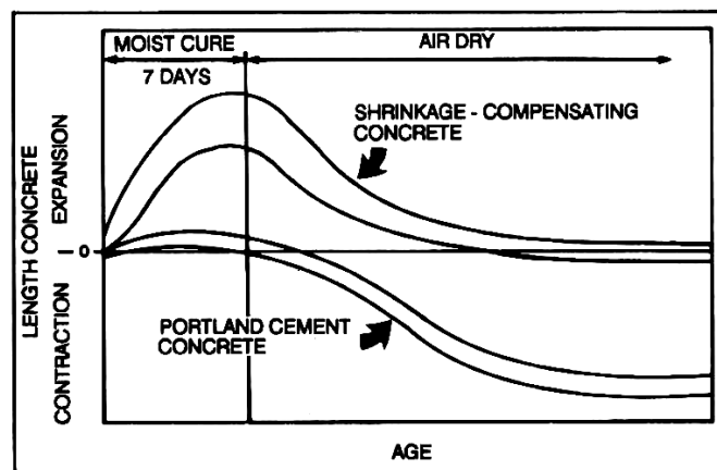
Figure 2.1: Typical length change characteristics of shrinkage compensating and portland cement concretes ( Gruner and Plain 1993 )
