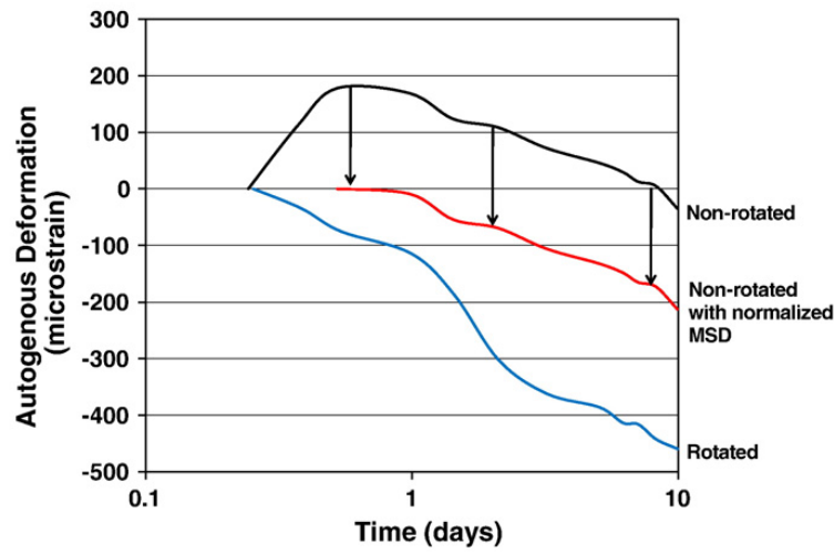
Figure 4.5: Comparison of rotated and non-rotated autogenous testing( Mohr and Hood 2010 )
