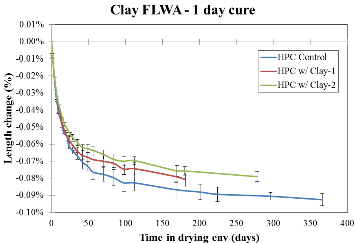
Figure 5.8: Drying shrinkage results, 1 day cure (clay FLWA mixtures)
