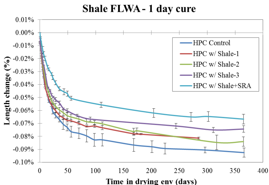
Figure 5.11: Drying shrinkage results, 1 day cure (shale FLWA mixtures)
