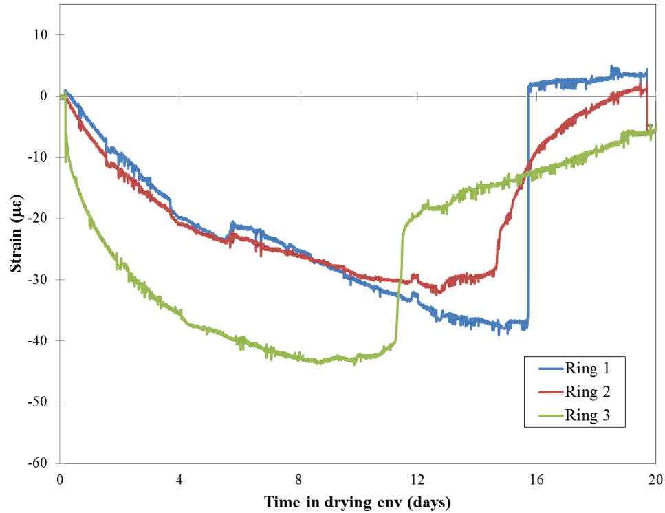
Figure 5.19: Restrained shrinkage, HPC w/ SRA - 14 day cure
