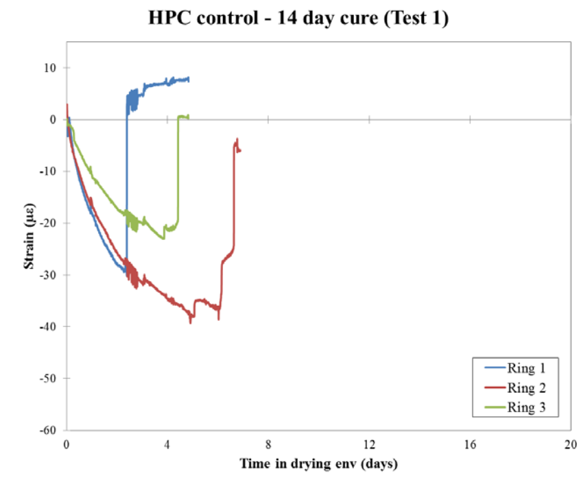
Figure 5.17: Restrained shrinkage, HPC control - 14 day cure (Test 1)
