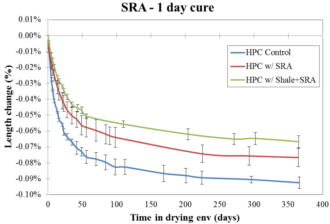
Figure 5.14: Drying shrinkage results, 1 day cure (SRA mixtures)
