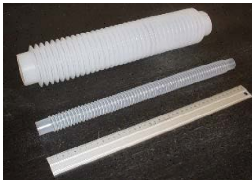
Figure 4.6: Larger corrugated tubes for testing autogenous strain of concrete( Bentz et al. 2009 )
