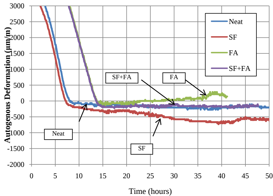
Figure 5.4: Effect of SCMs on autogenous deformation (w/cm = 0.37 w/cm, 20 °C)
