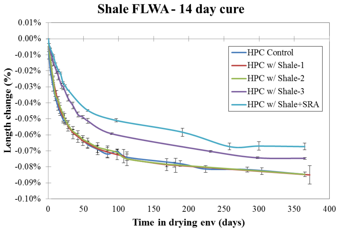
Figure 5.13: Drying shrinkage results, 14 day cure (shale FLWA mixtures)
