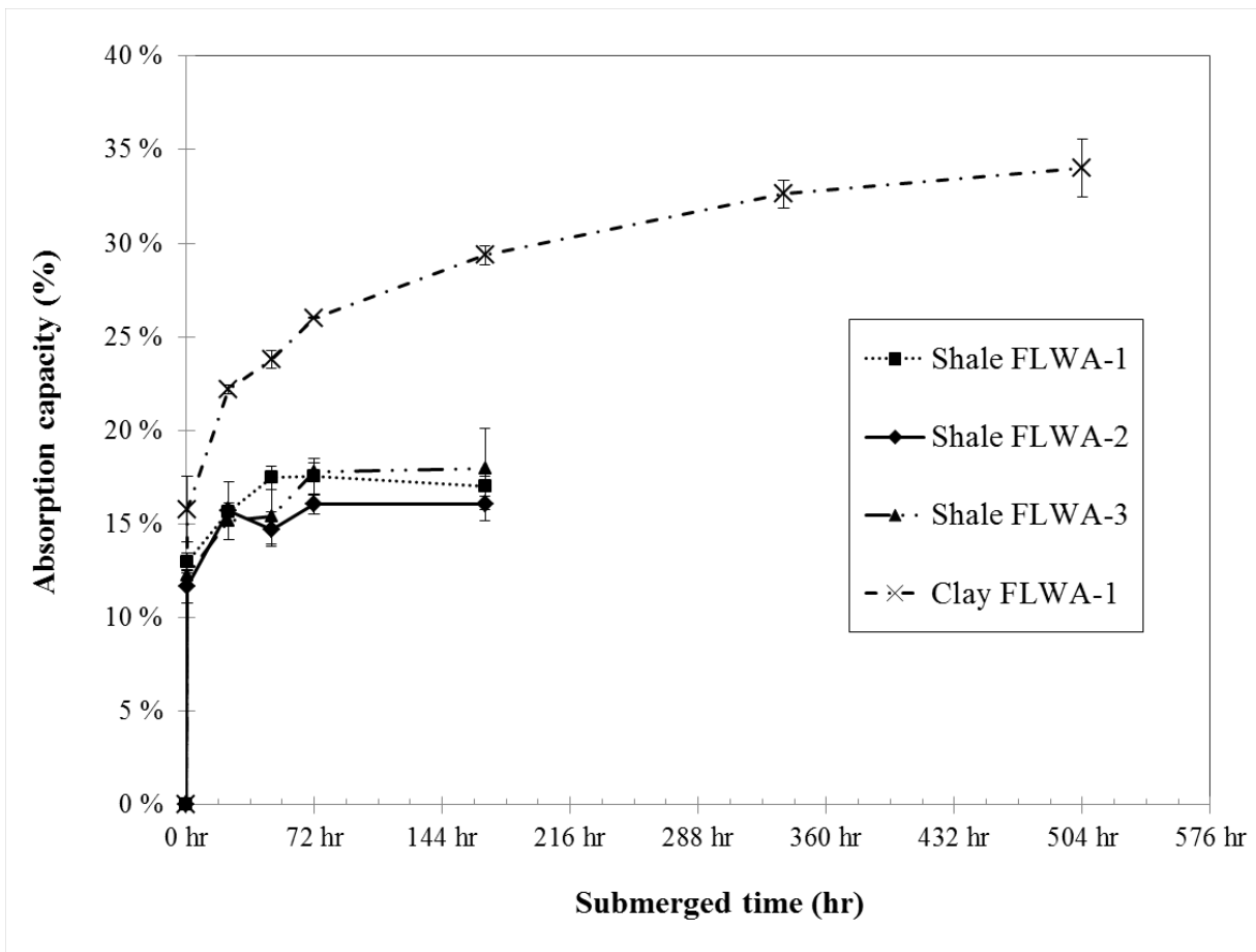
Figure 5.1: Absorption capacity of FLWAs
