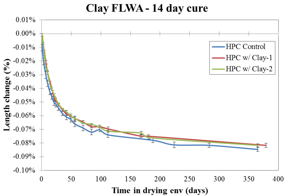
Figure 5.10: Drying shrinkage results, 14 day cure (clay FLWA mixtures)
