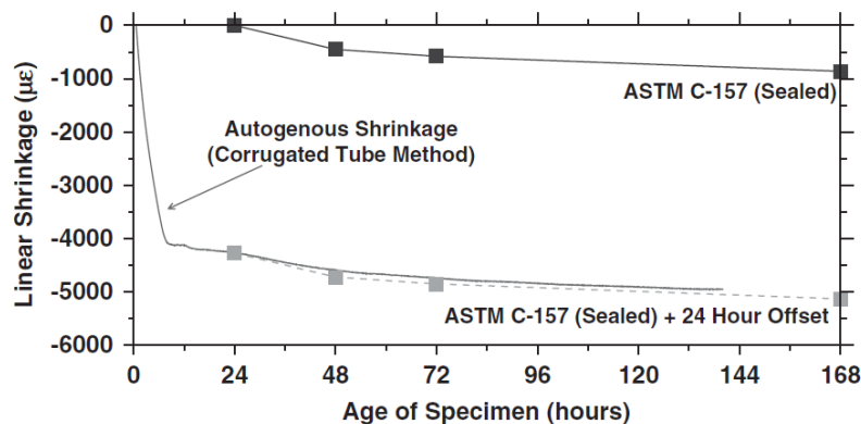
Figure 4.7: Comparison of autogenous shrinkage measured in sealed specimens using ASTM C157 (beginning at 24 h) and corrugated mold procedure (beginning immediately after mixing) for a w/cm = 0.30 mixture ( Sant et al. 2006 )
