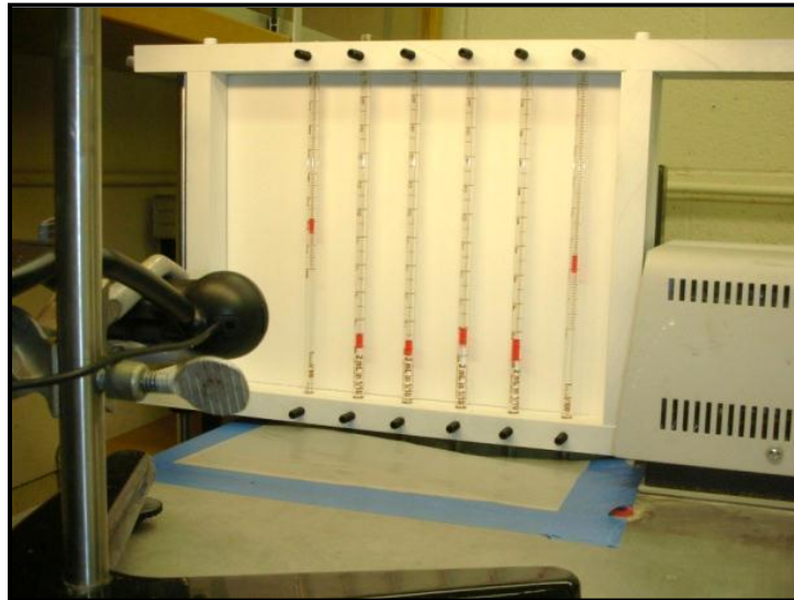
Figure 4.10: Automated chemical shrinkage test set-up( Ideker 2008 )
