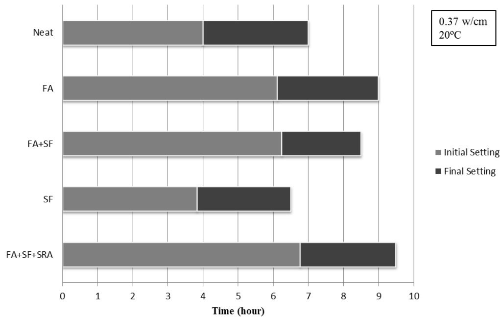
Figure 5.3: Vicat setting time results for OPC systems (w/cm = 0.37, 20 °C)
