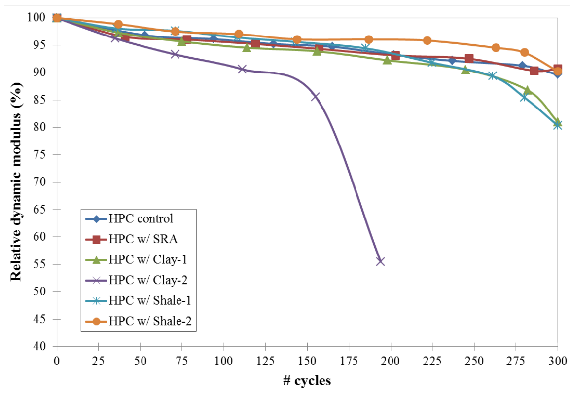
Figure 5.25: Freeze-thaw testing, relative dynamic modulus
