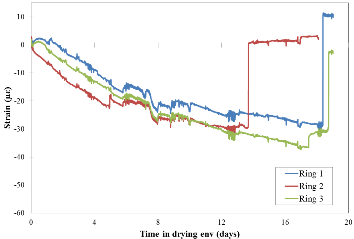
Figure 5.22: Restrained shrinkage, HPC w/ SRA - 3 day cure
