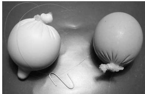
Figure 4.1: Polyurethane membrane (left) and latex membrane (right) filled with cement paste ( Lura and Jensen 2007 )
