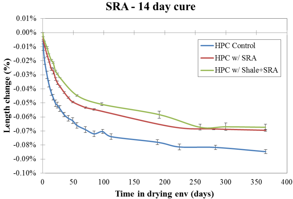
Figure 5.16: Drying shrinkage results, 14 day cure (SRA mixtures)
