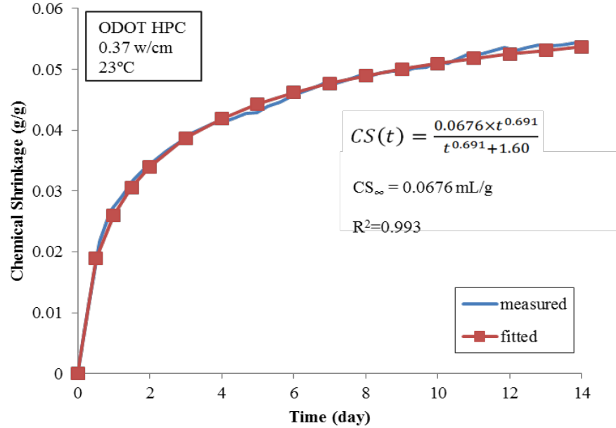
Figure 5.7: CS development curve, HPC w/cm = 0.37 at 23 °C isothermal (Fu et al. 2012)
