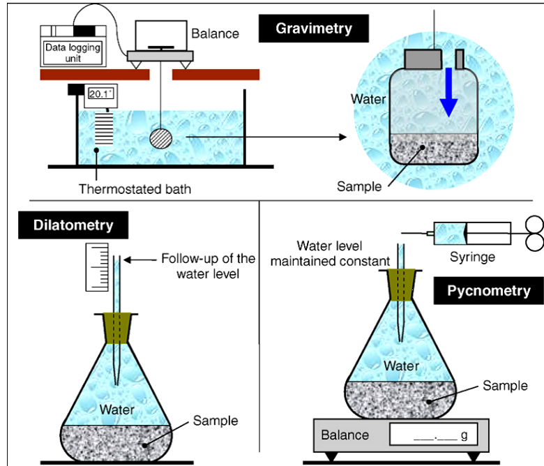
Figure 4.9: Chemical shrinkage measurement methods (Bouasker et al. 2008)
