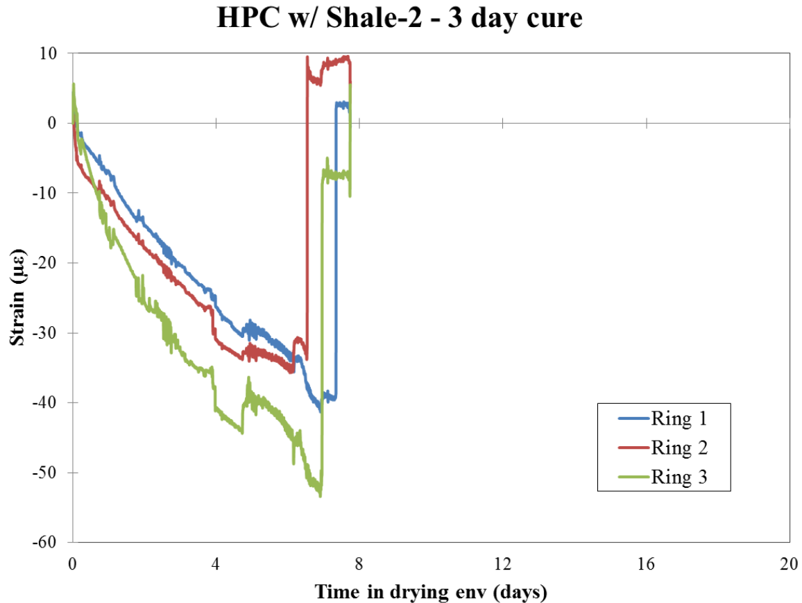
Figure 5.23: Restrained shrinkage, HPC w/ Shale-2 - 3 day cure
