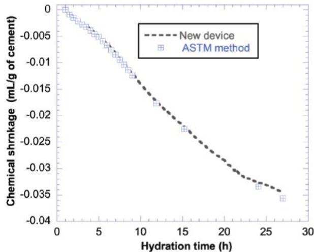
Figure 4.13: Comparison of CS results for pressure method and ASTM C1608(Peethamparan et al. 2010)
