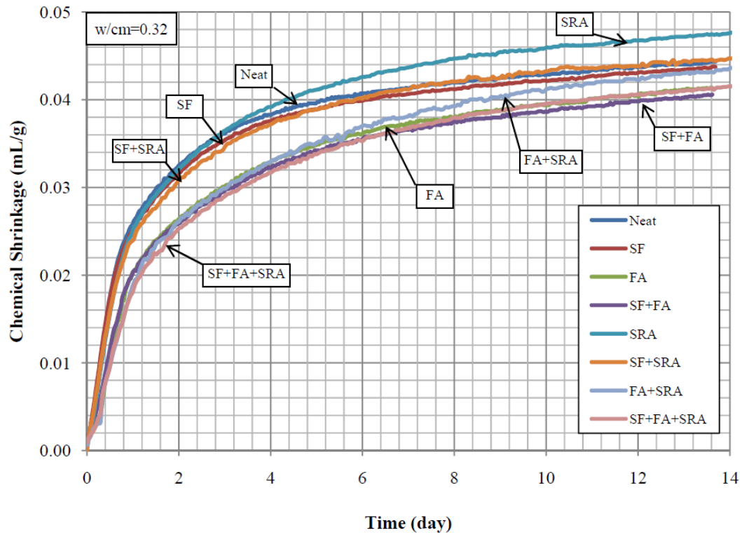
Figure 4.11: Typical chemical shrinkage results for OPC mixtures at 20 °C ( Fu 2011 )
