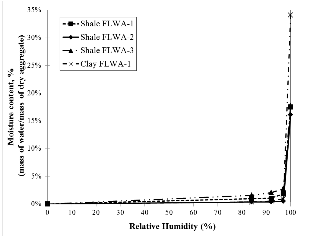
Figure 5.2: Desorption testing of FLWA
