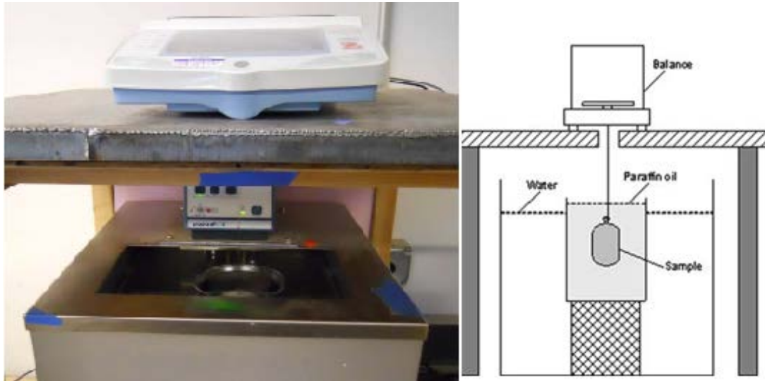
Figure 4.2: Experimental set-up for membrane method to test autogenous strain for cement paste ( Fu 2011; Lura and Jensen 2007 )
