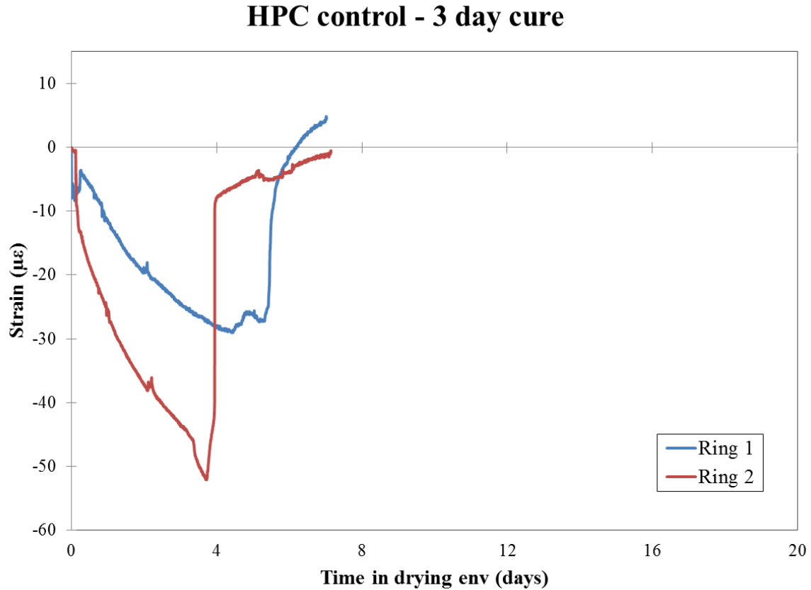
Figure 5.21: Restrained shrinkage, HPC control - 3 day cure
