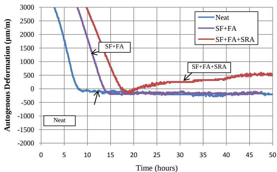
Figure 5.5: Effect of SRAs on autogenous deformation (w/cm = 0.37, 20 °C)
