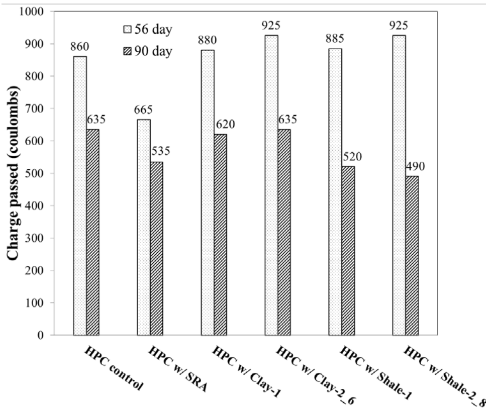
Figure 5.24: RCPT results
