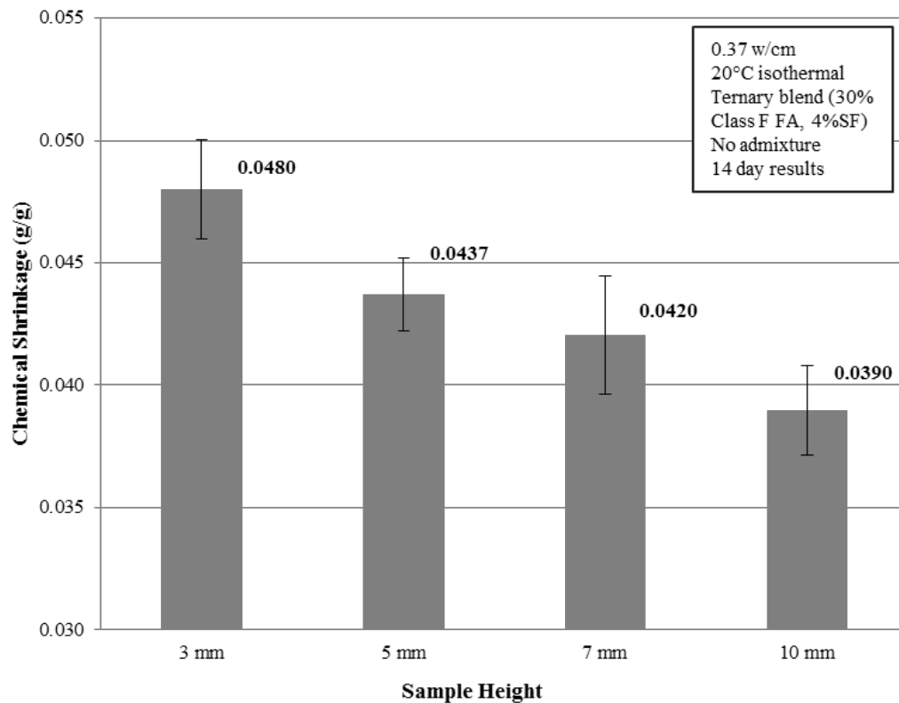
Figure 5.6: CS depercolation study (Fu et al. 2012)
