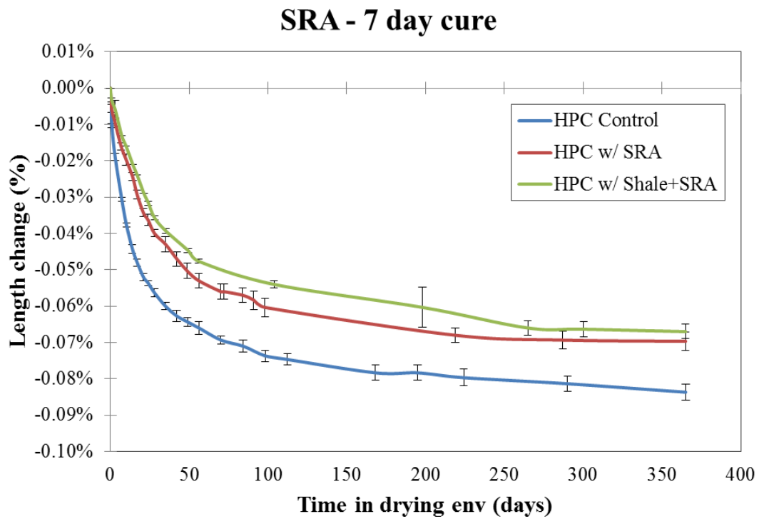
Figure 5.15: Drying shrinkage results, 7 day cure (SRA mixtures)
