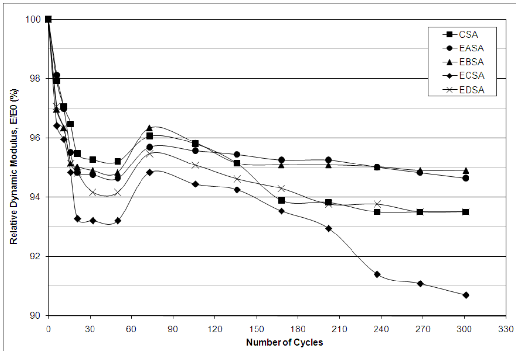
Figure 5.6 - Relative Dynamic Modulus for Mixtures Cured using Steam Curing Method A
