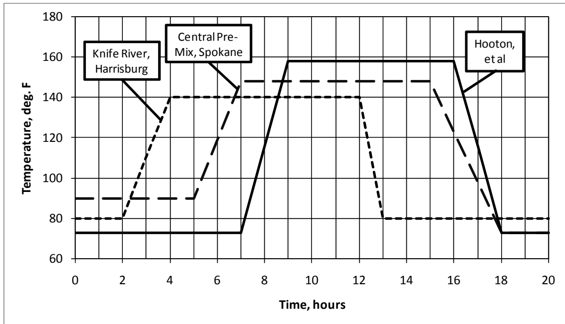
Figure 4.2 - Contractor and Laboratory Steam Curing Regimes
