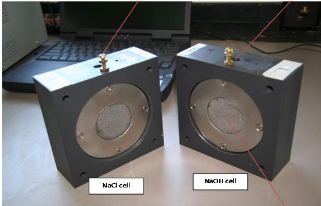
Figure 4.10 - Chloride Ion Permeability Specimen Cell
