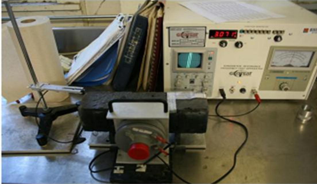
Figure 4.18 - Fundamental Transverse Frequency Measurement
