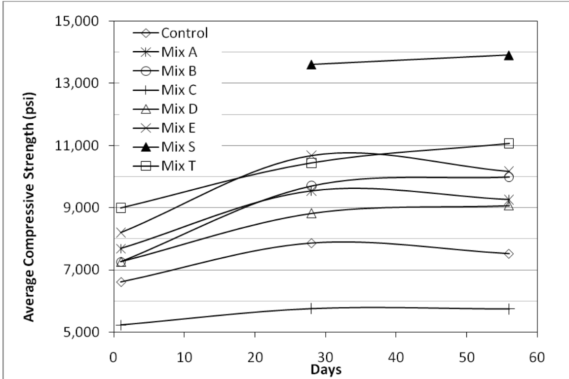
Figure 5.16 - Evolution of Compressive Strength of the Mixtures Tested in Phase II
