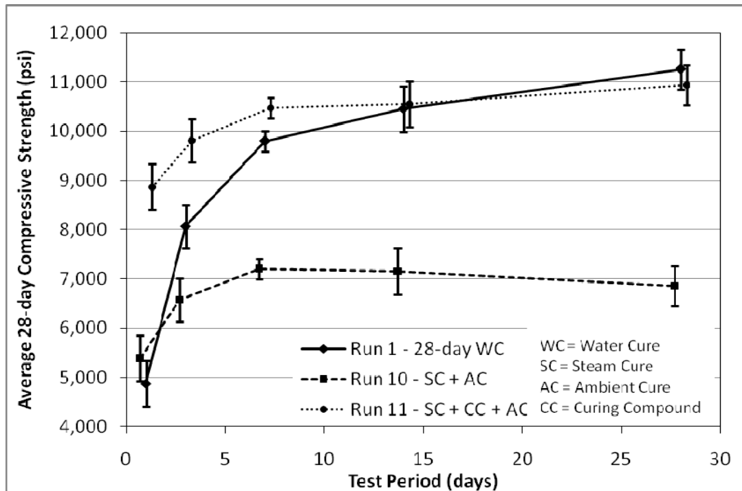
Figure 5.15 - Strength Gain of Steam-Cured and Continuously Water-Cured Specimens
