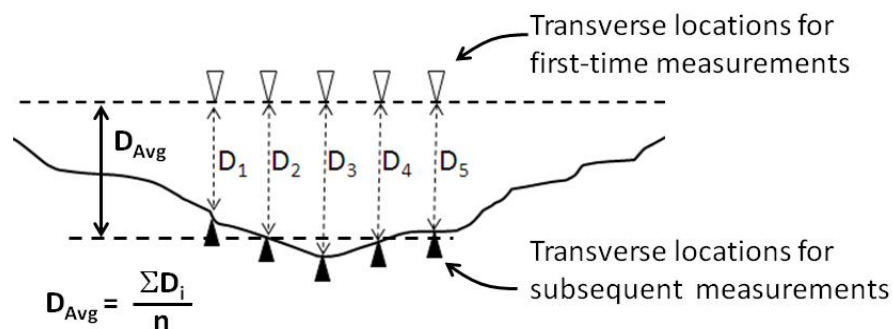
Figure F.3: Determination of the Average Wear Depth within a Single Wheel Path
