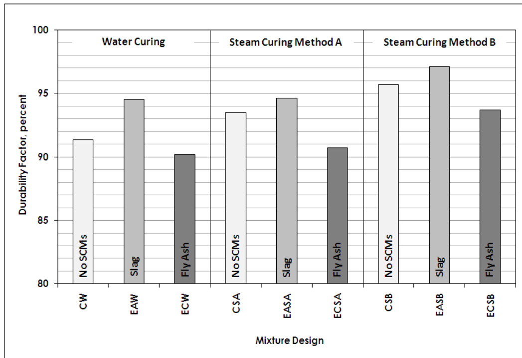
Figure 5.8 - Durability Factors of Mixtures with River Gravel
