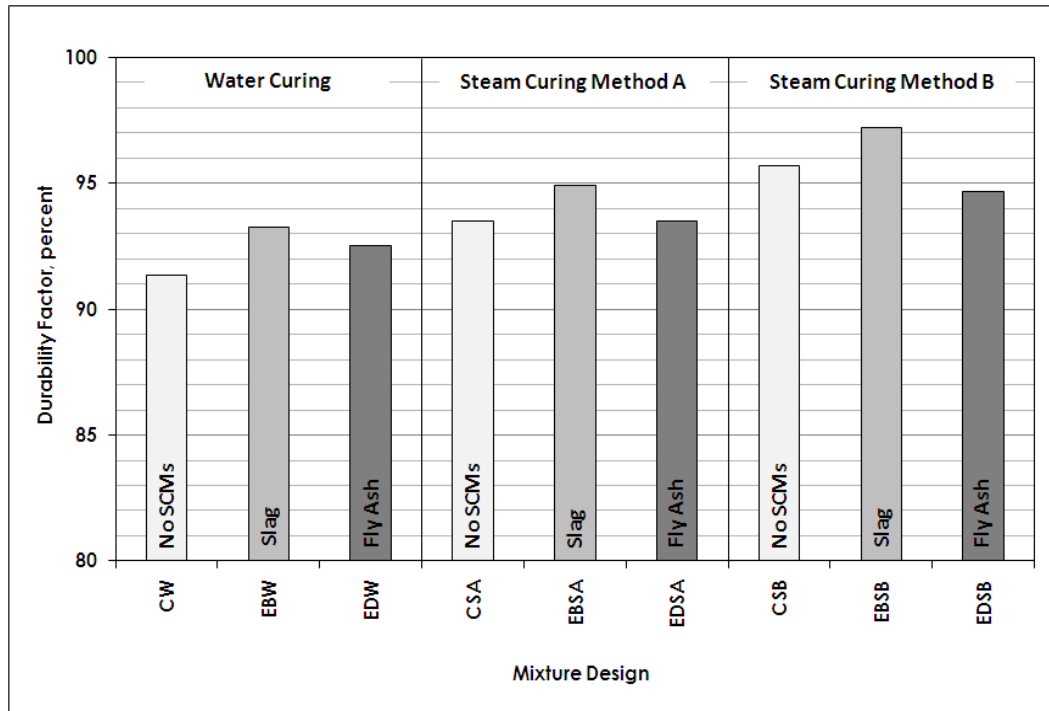
Figure 5.9 - Durability Factors of the Control Mixture and Those with Crushed Rock
