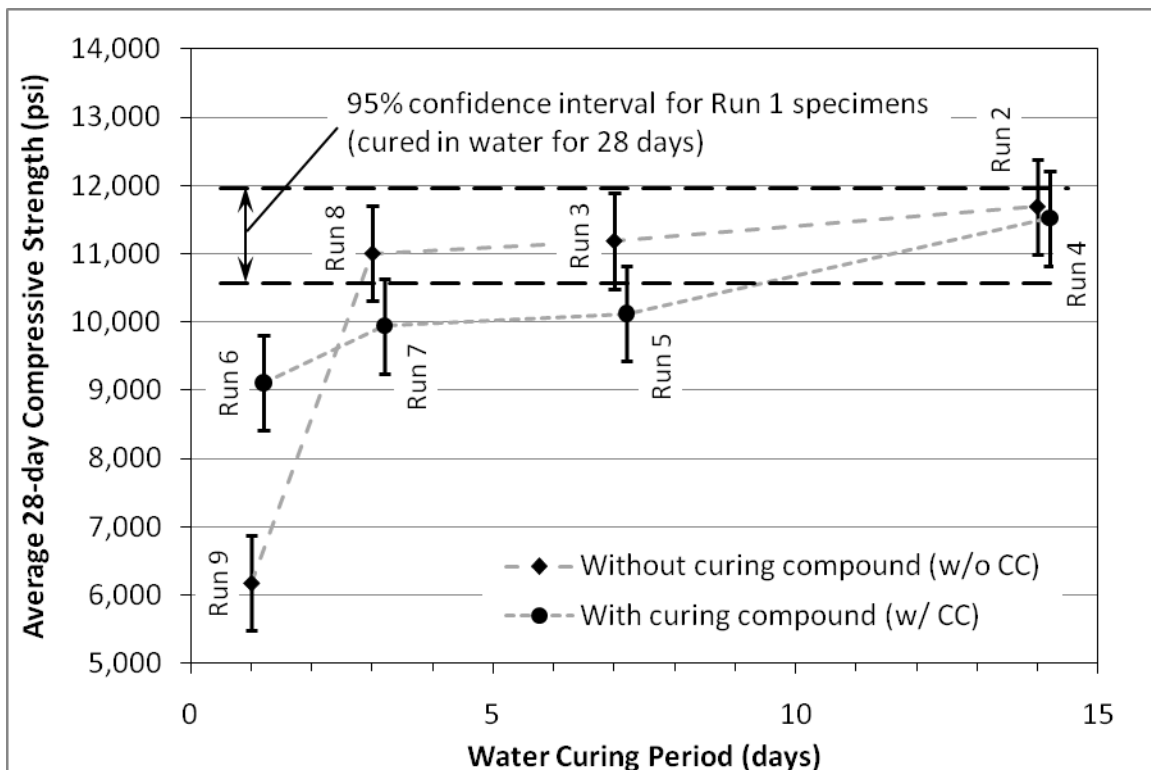
Figure 5.14 - 28-day Strengths of Water-Cured Specimens
