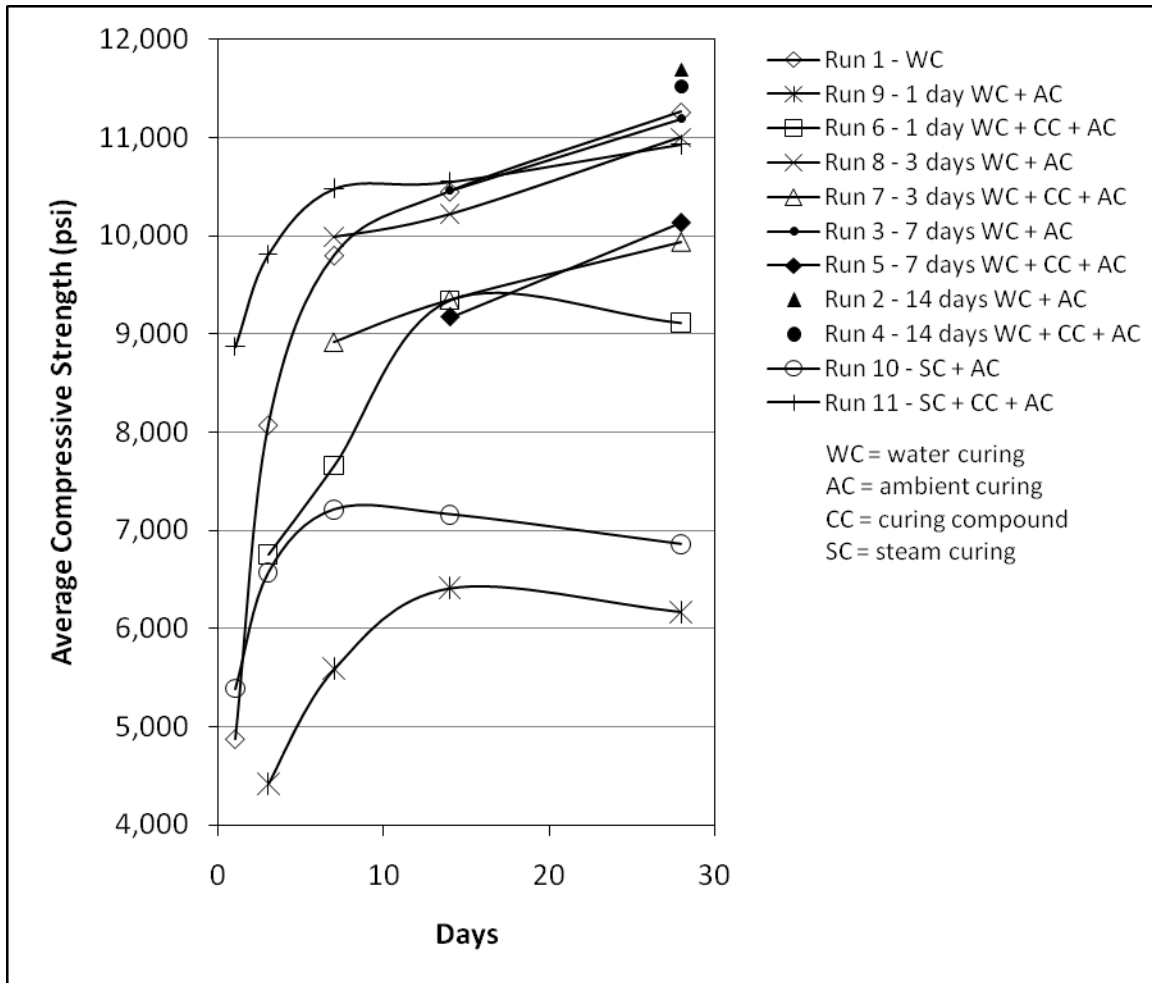
Figure 5.13 - Evolution of Strength due to Curing Regimes Investigated in the Pilot Study
