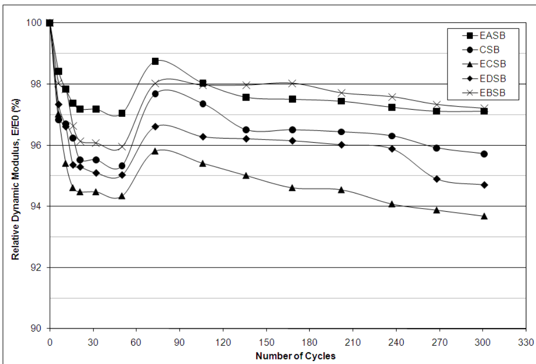
Figure 5.7 - Relative Dynamic Modulus for Mixtures Cured using Steam Curing Method B
