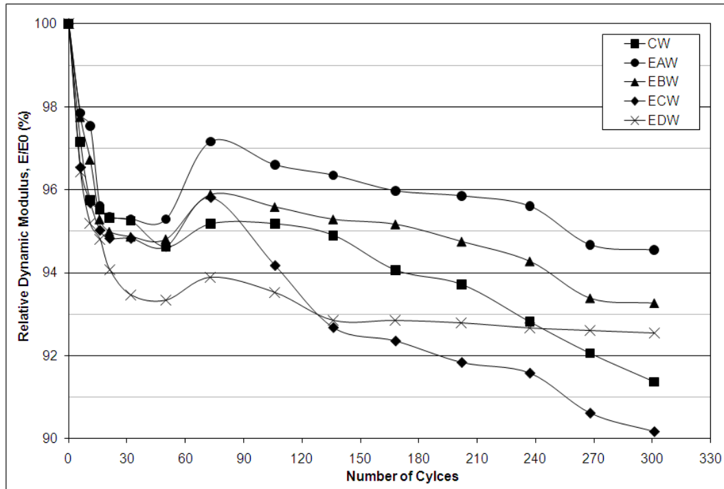
Figure 5.5 - Relative Dynamic Modulus for Mixtures Cured in Water
