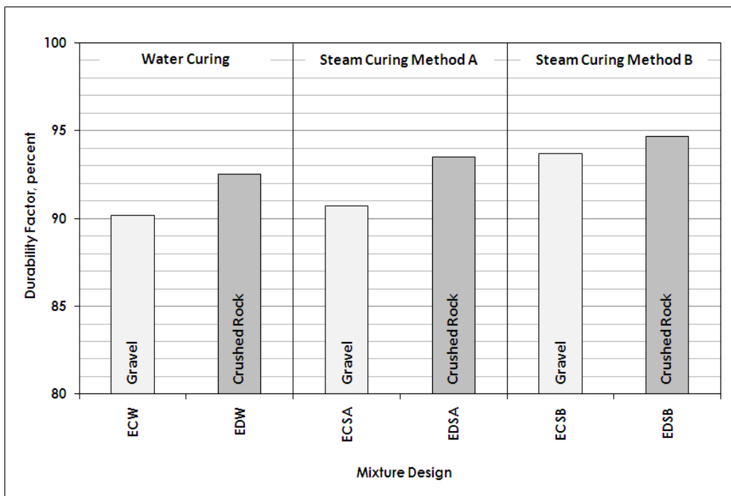
Figure 5.11 - Durability Factors of Mixture with Fly Ash
