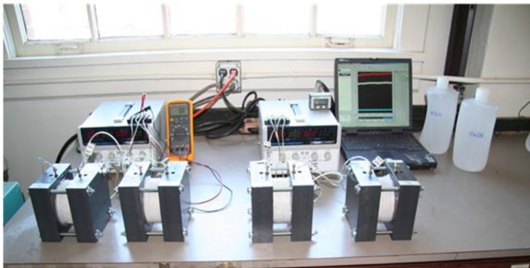
Figure 4.11 - Setup for the Rapid Chloride Penetration Test
