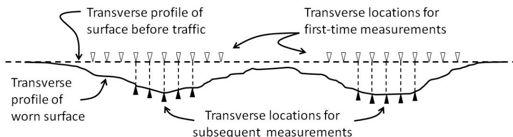
Figure F.2: Conceptual Layout of Surface Profile Measurement Locations
