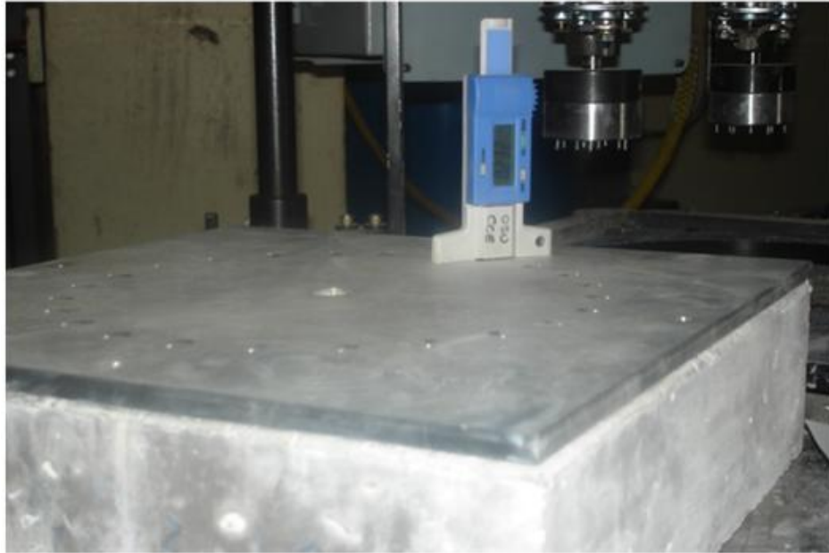
Figure 4.4 - Measurement of Wear Depth using a Depth Micrometer
