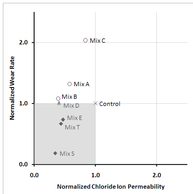
Figure 5.17 - Mixture Selection Chart based on Relative Performance
