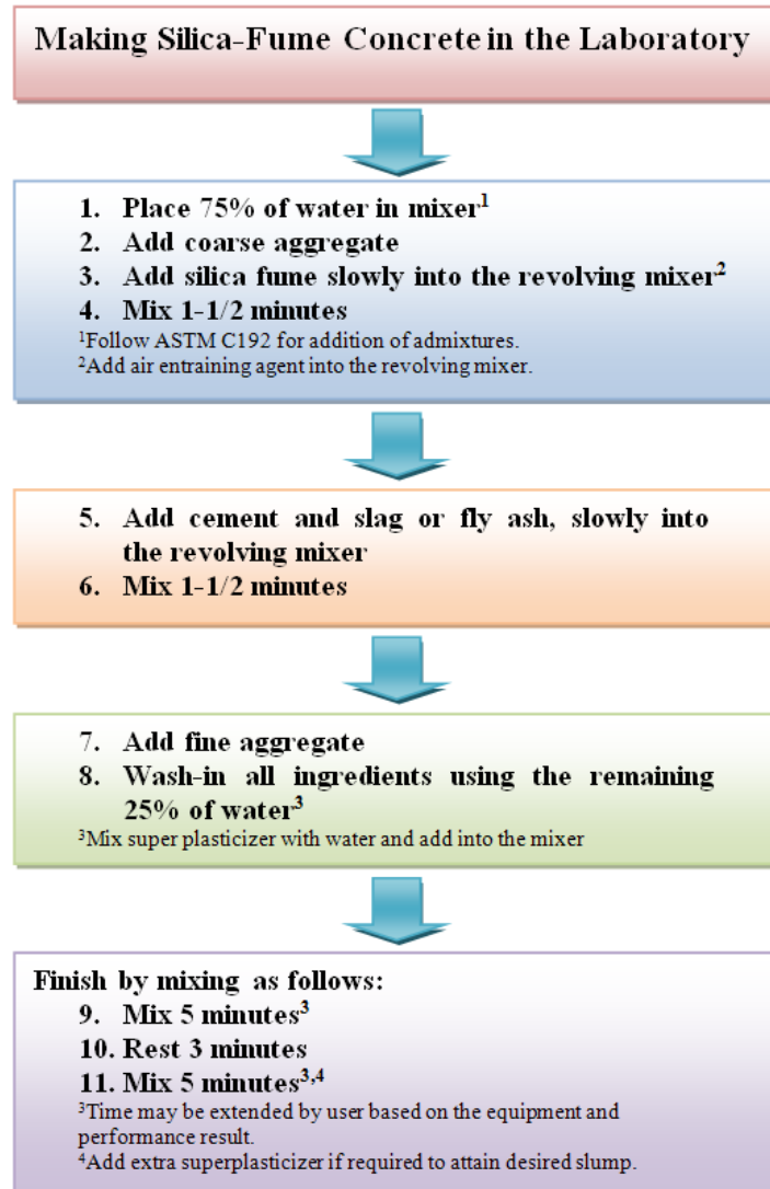
Figure 4.1 - Flow Chart for Mixing Procedure (adapted from 37)
