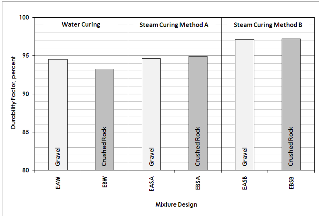
Figure 5.10 - Durability Factors of Mixtures with Slag
