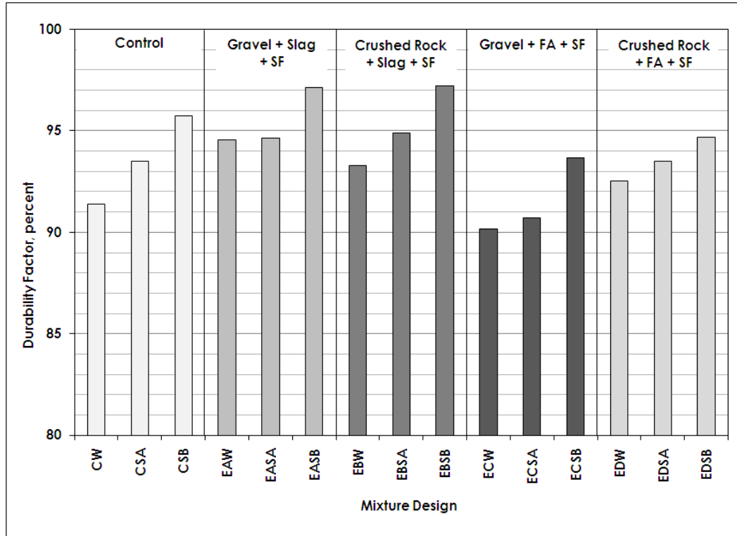
Figure 5.12 - Effect of Curing Method on the Durability Factor of Various Mixtures
