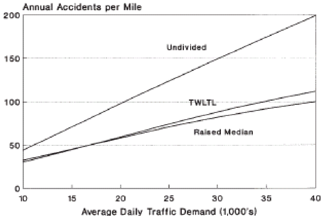
Figure 2.6: Predicted Average Crash Frequency Comparison
