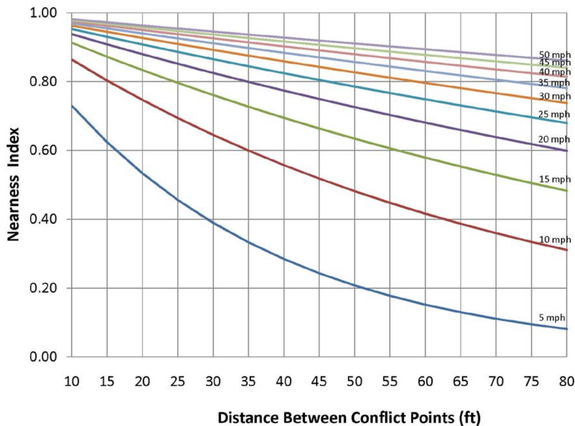
Figure 6.2: Nearness Index
