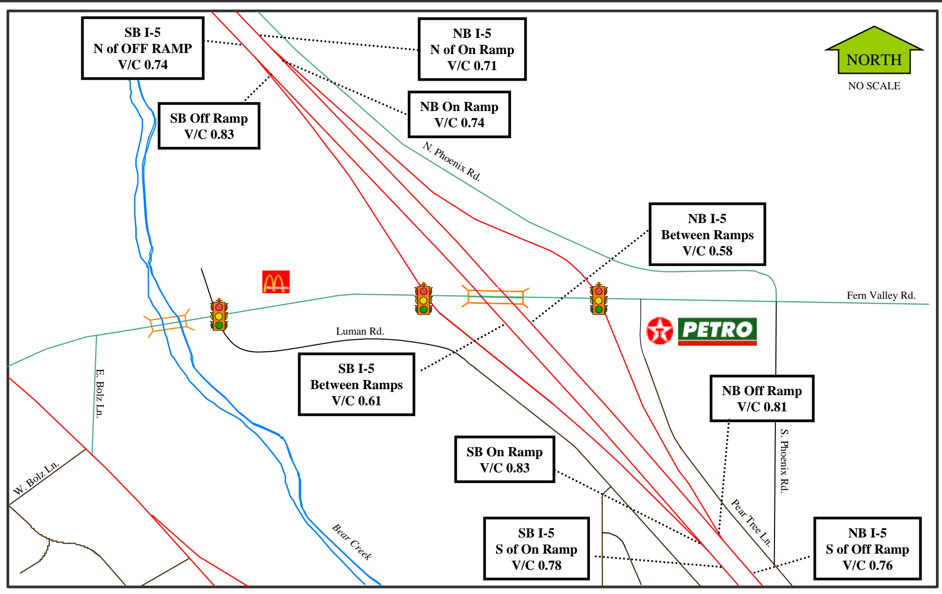
Fern Valley Interchange – 2030 Future No-Build V/C Ratios
