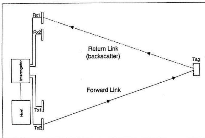
Figure 2.1: MicroStamp 4000 System (courtesy of Micron Communications, Inc.)
