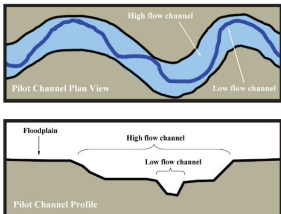
Figure 6. Plan and profile views of the Anderson Creek pilot channel illustrating channel layout and high and low flow channels.
