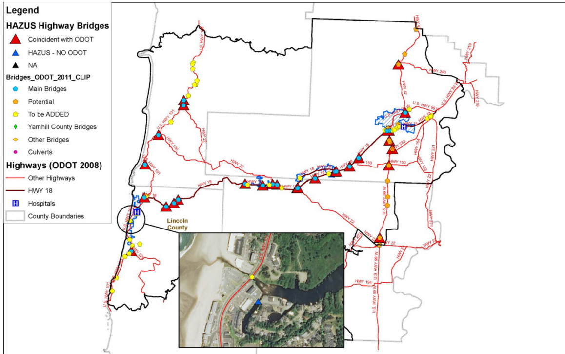
Figure 28. Project area bridge inventory discrepancies between the Hazus bridge database and the ODOT bridge database. The photo inset shows the single span bridge east of the D River bridge where ownership could not be determined. This is not a damage map.
