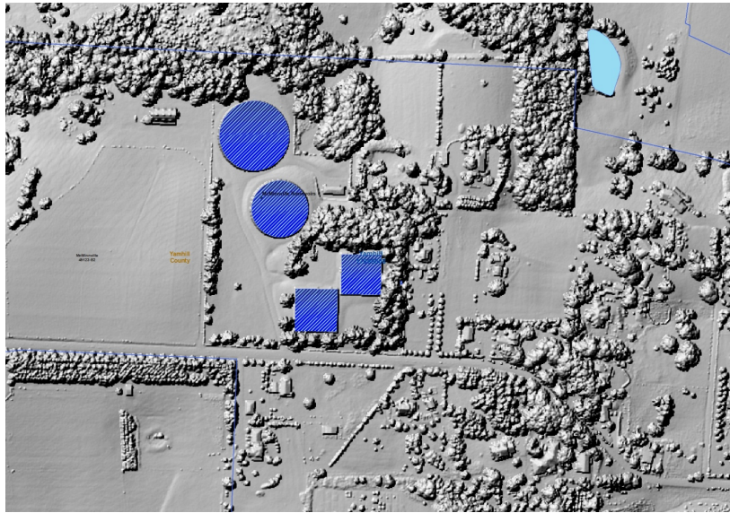
Figure 26. McMinnville Water and Light Fox Ridge Reservoirs (identified in blue) and control building (gray rectangular building to the right of the lower round tank) on a lidar basemap.
