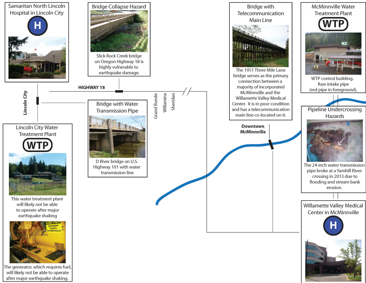
Figure 42. Schematic of critical facilities and pathways in the project area include the two hospitals, two water treatment plants, and the highways and pipelines connecting them. The blue line is the Yamhill River.
