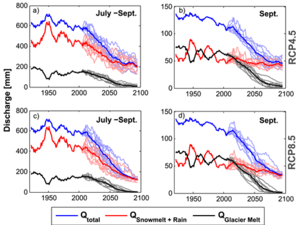
Figure 14 Historical and future (a and c) dry season (July to September) and (b and d) September discharge volume ( Q ) of Eliot Creek, a tributary of the Hood River, for (a and b) lower (RCP4.5) and (c and d) higher (RCP8.5) emissions scenarios. (Figure Source: Implications of decadal to century scale glacio-hydrological change for water resources of the Hood River basin, OR, USA, Volume: 30, Issue: 23, Pages: 4314-4329, First published: 07 April 2016, DOI: https://doi.org/10.1002/hyp.10872 )
