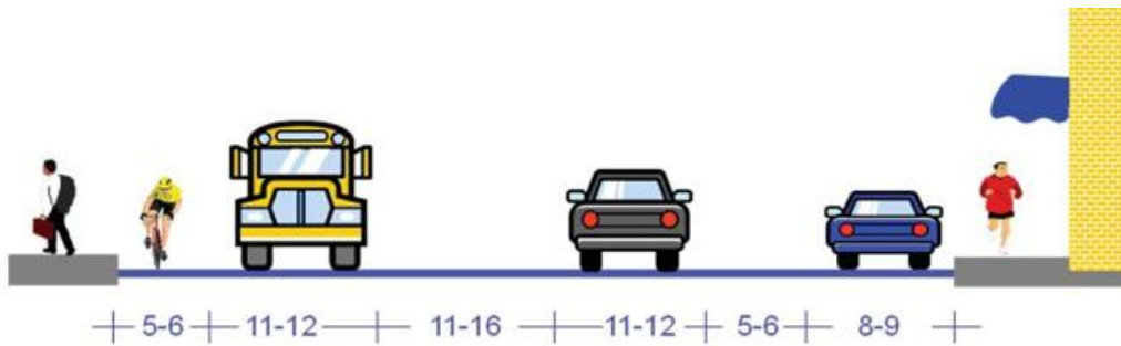
Example cross-section with two-way left turn lane, bicycle lanes and parking
