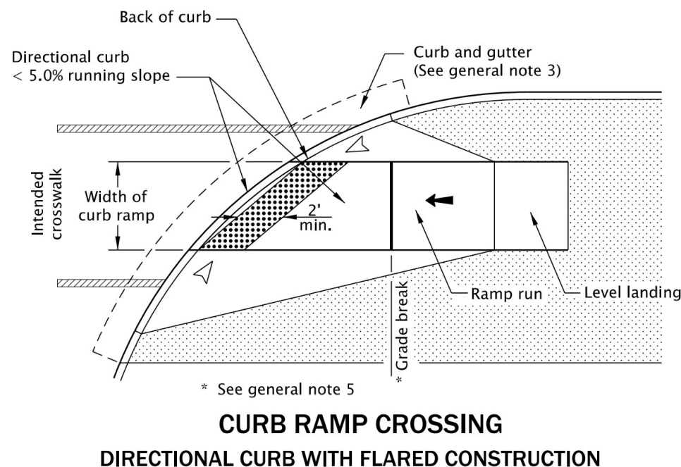
Figure 800-58: Directional Curb with Flared Construction
