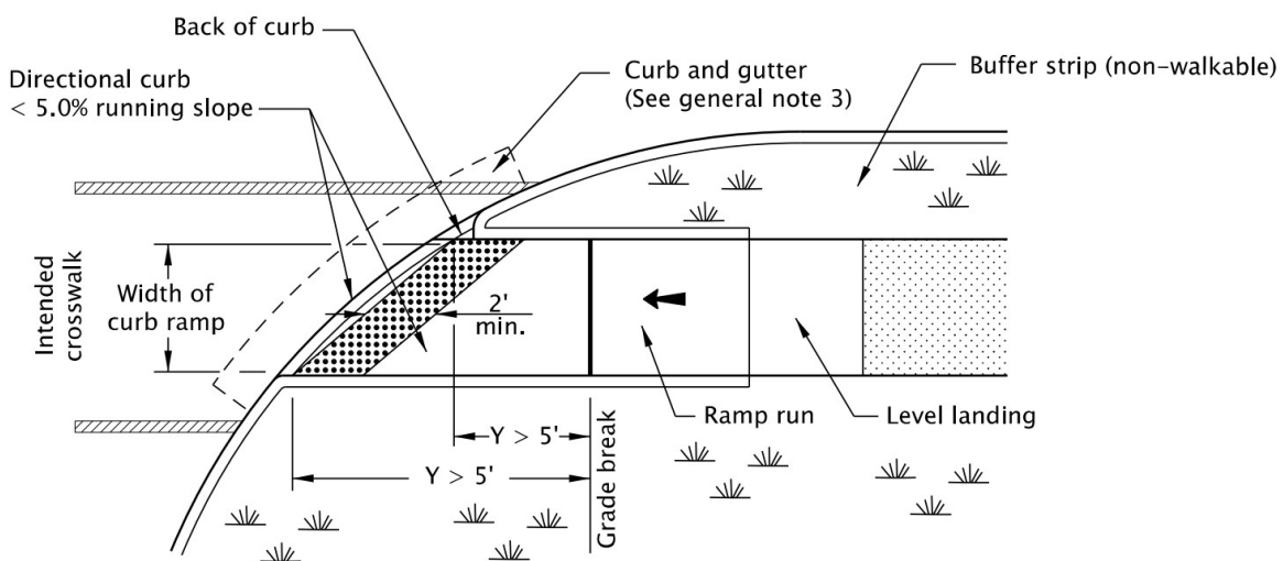
Figure 800-60: Directional Curb with Grade Break Larger than 5 Feet and No Flare
