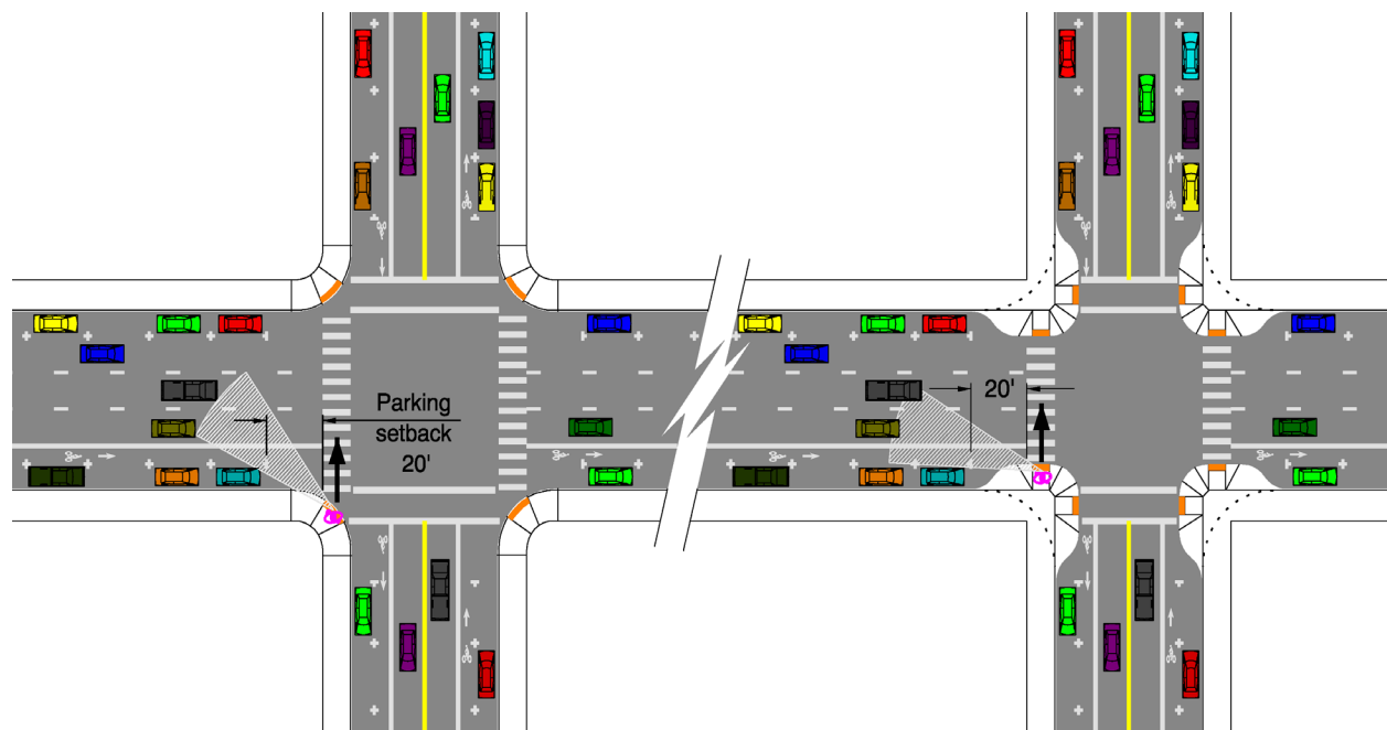
Figure 800-69: Sight Lines with Curb Extensions
