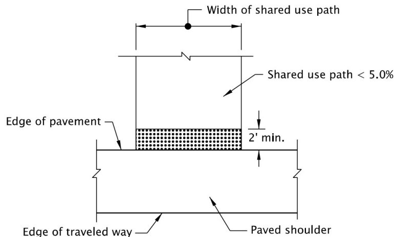
Figure 800-53: Detectable warning surface with No Curb Zone (Source: Standard Dwg. RD904)
