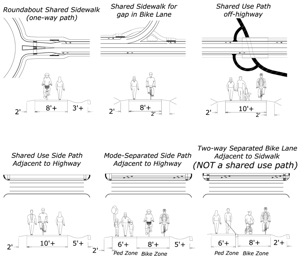
Figure 800-72: Types of Shared Use Paths
