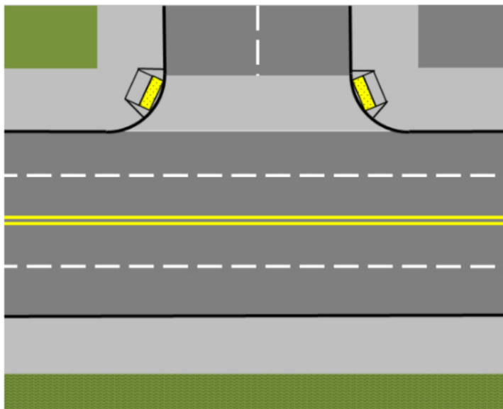
Figure 800-63: Detectable Warning Surface at Curb Radii Driveway
