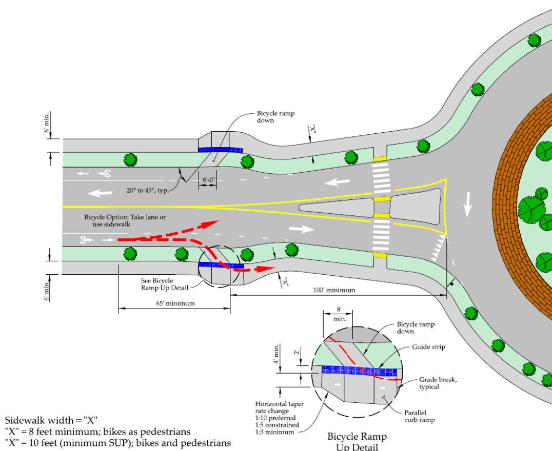
Figure 800-73: Bike Ramp Connection to Sidewalk on Roundabout Approach Street
