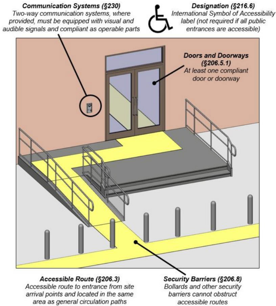
Figure 800-50: ADA Building Ramps Accessible Routes Illustration, source US Access Board
