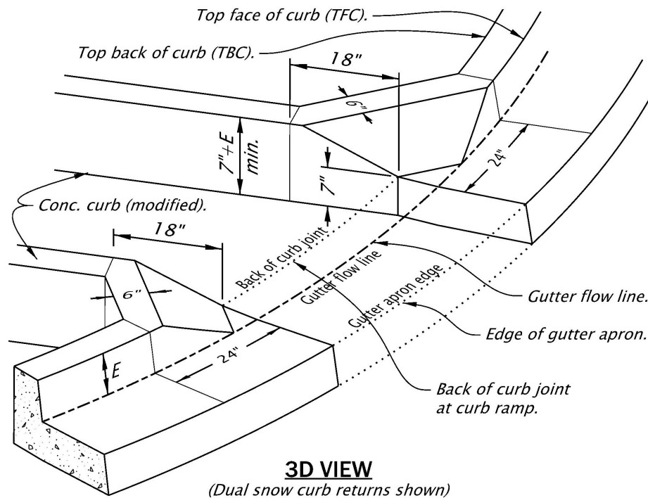
Figure 800-48: Snow Curb Return
