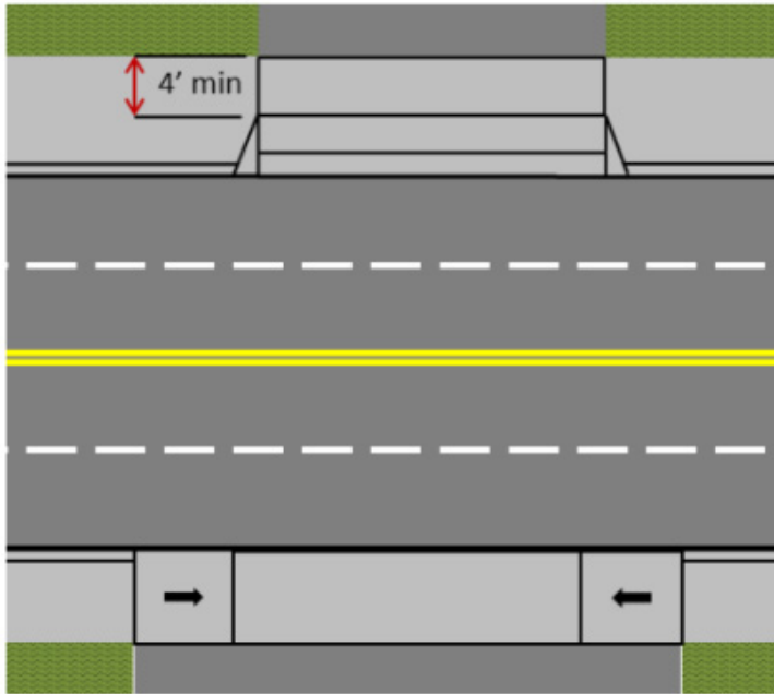
Figure 800-63: Detectable Warning Surface at Curb Radii Driveway
