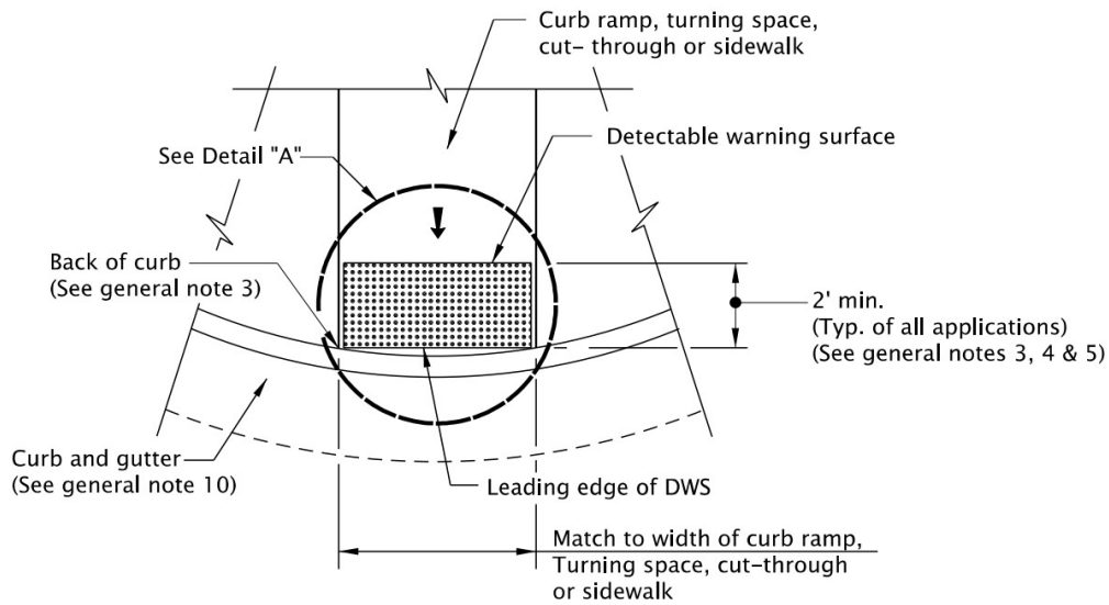
Figure 800-54: Detectable warning surface at Curb Ramp
