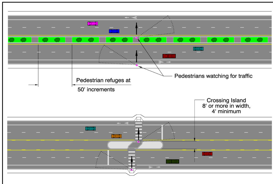
Figure 800-67: Continuous Raised Median versus Cut-Through Crossing Island
