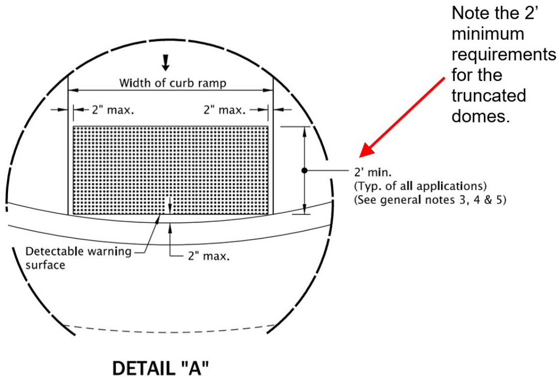
Figure 800-55: Detectable Warning Surface Maximum Gap Space Detail
