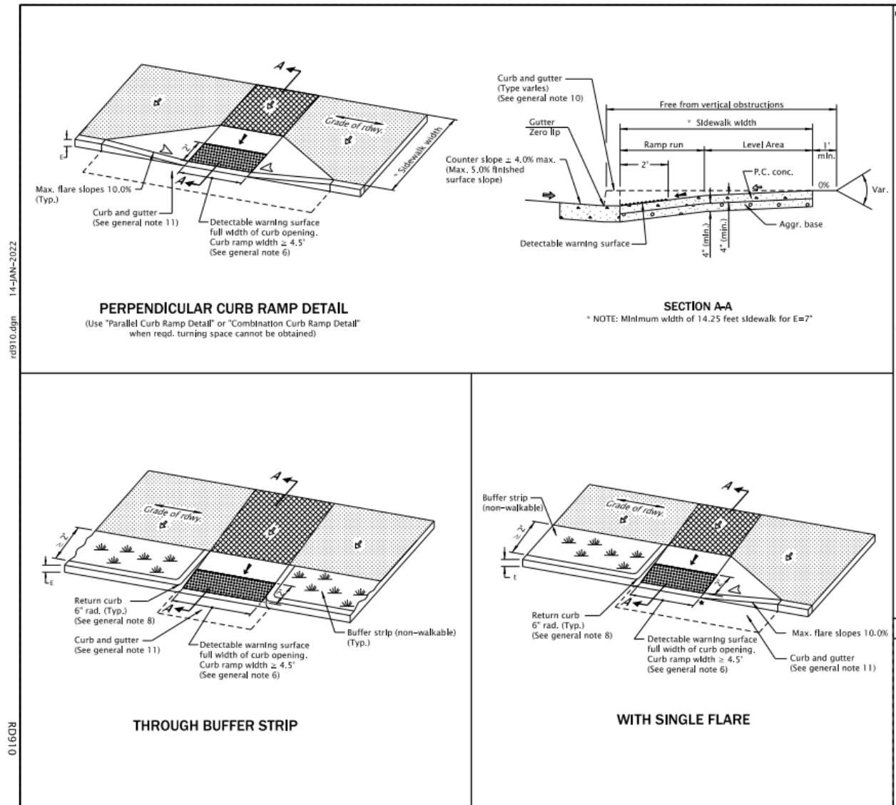
Figure 800-33: Perpendicular Curb Ramp System
