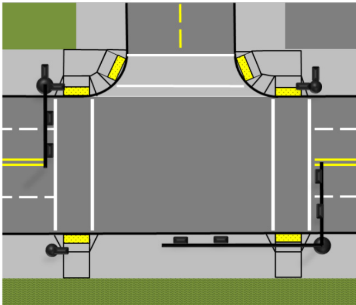
Figure 800-65: Signalized Driveway Example 2
