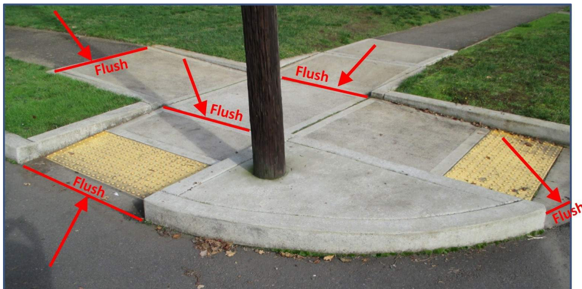
Figure 800-47: Locations Where Lips Might Occur
