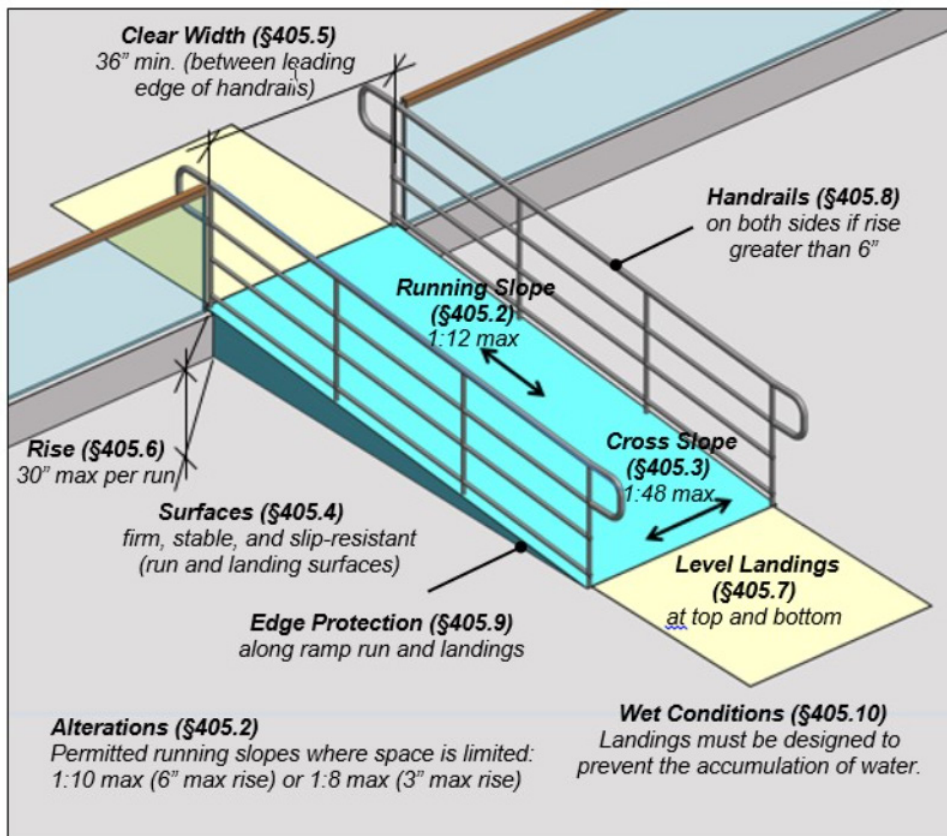
Figure 800-51: ADA Building Ramps Illustration, Source US Access Board and CFR
