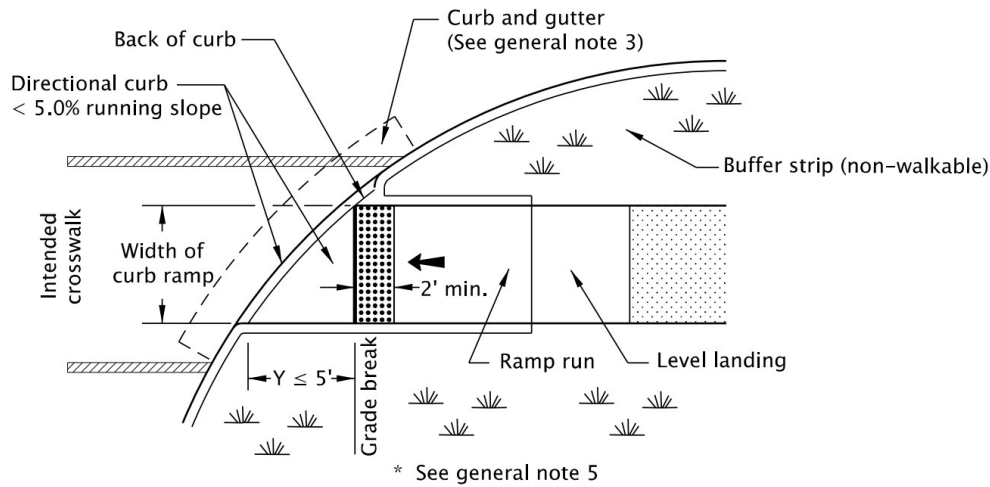
Figure 800-59: Directional Curb with Grade Break Less than 5 Feet and No Flare
