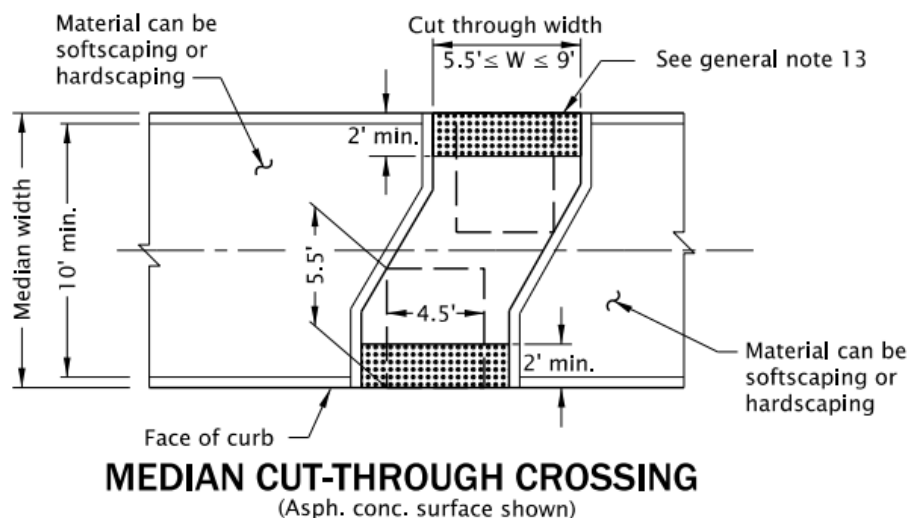
Figure 800-68: Angled Median Cut-Through Crossing
