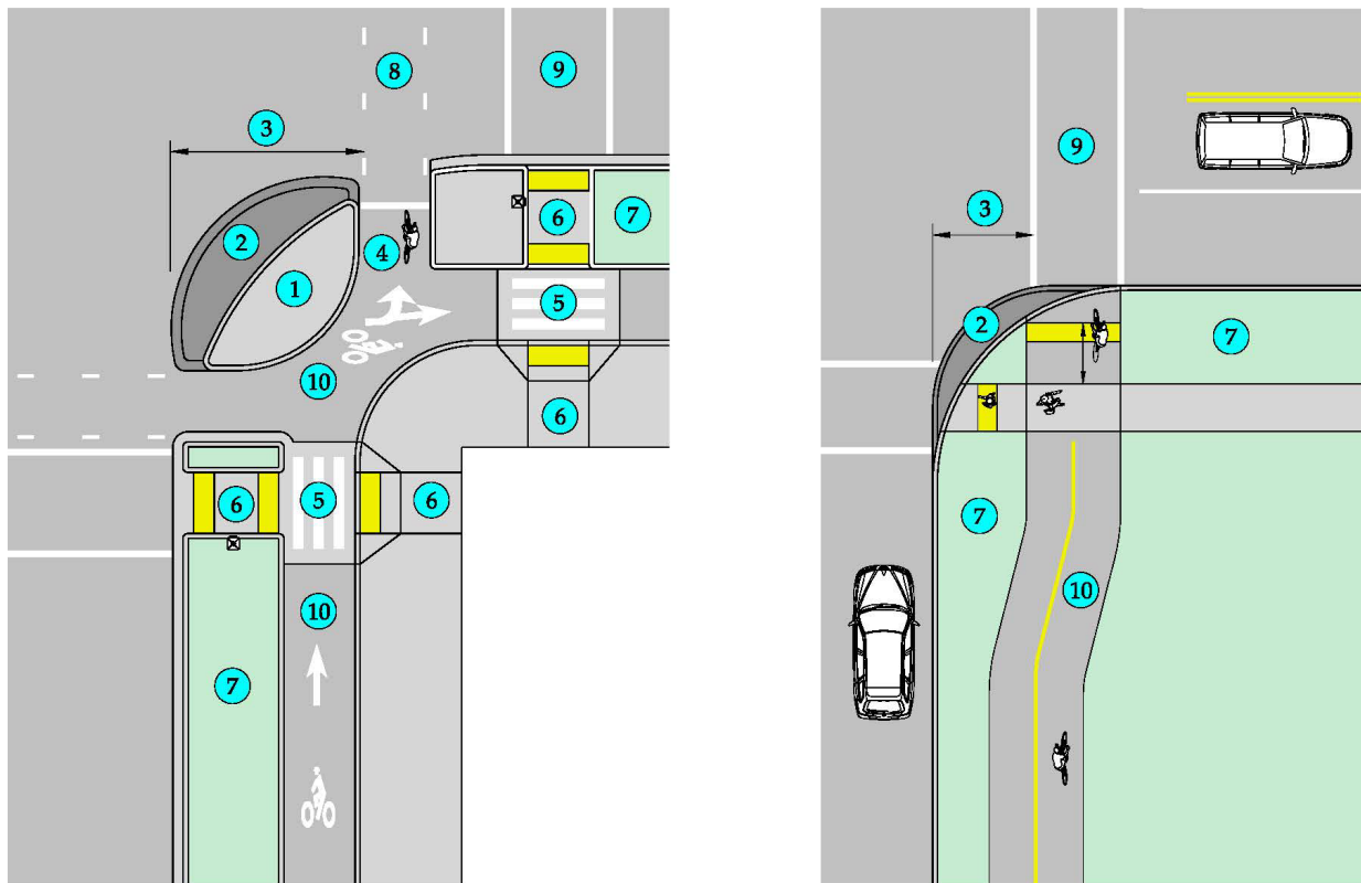
Figure 900-20: Protected Intersection Design for Separated Bike Lanes and Side Paths
