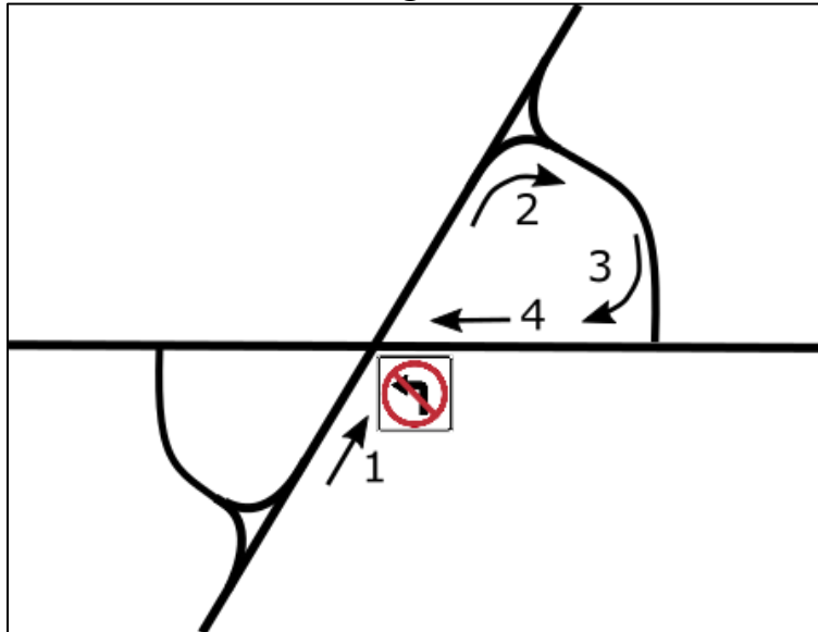
Exhibit 10-13 At-Grade Jughandle
