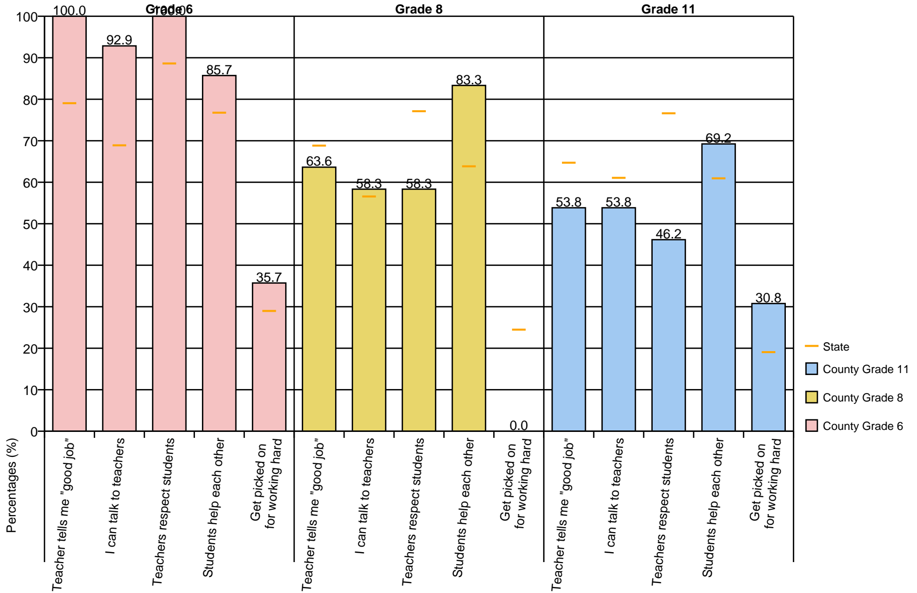
Figure 1: Supportive Atmosphere
