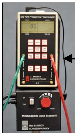
Fan control cable with Duct Blaster controller.
