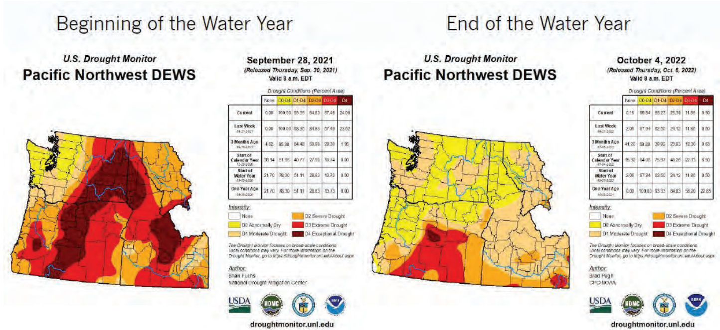
Figure 12. Average drought ratings for the Pacific Northwest from the beginning to the end of the previous "water year" (Sept 2021 to October 2022) relative to the average normal based on 115 years spanning from 1895 to 2010 (Western Regional Climate Center).
