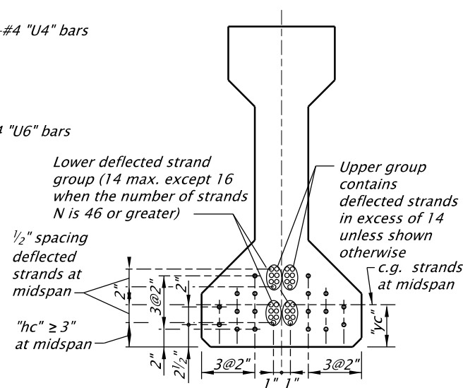
MIDSPAN SECTION
