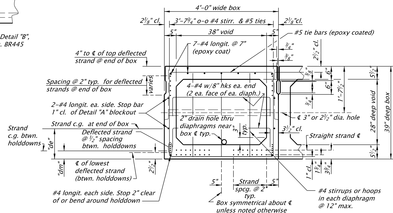
TYPICAL SECTION
