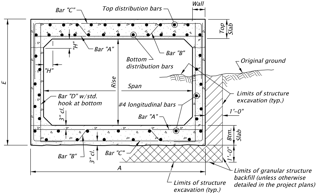
TYPICAL SECTION NONE
