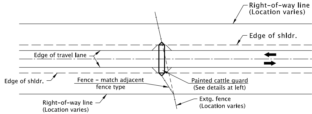
SINGLE INSTALLATION PLAN
