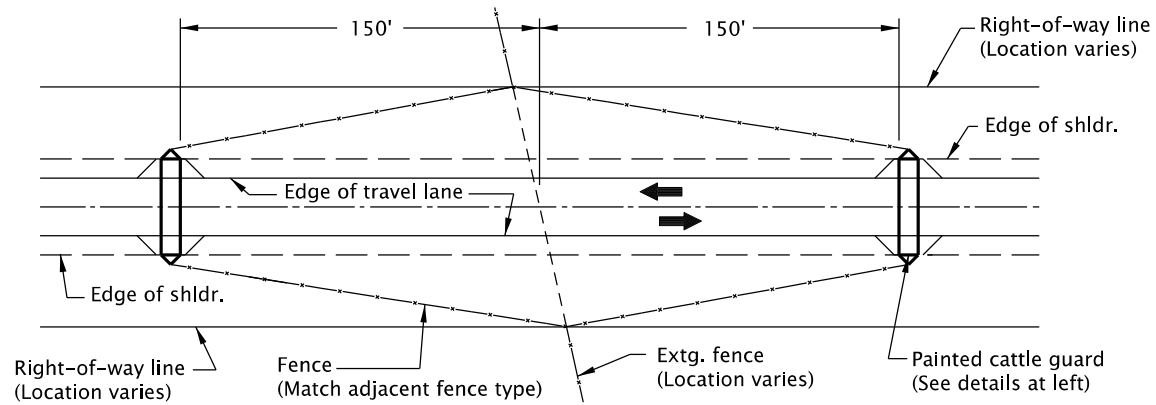
DOUBLE INSTALLATION PLAN
