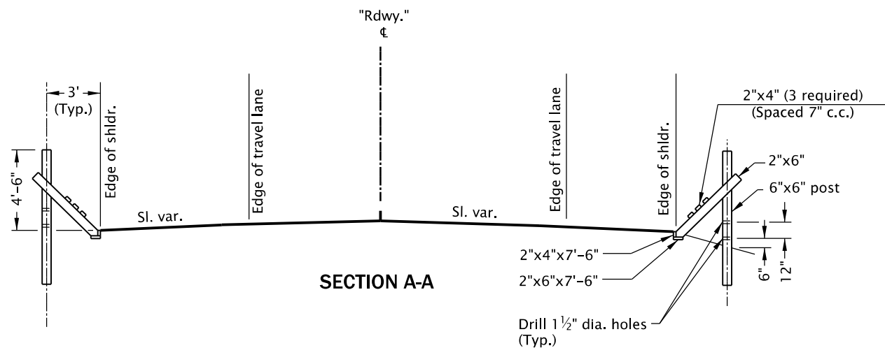
PAINTED CATTLE GUARD
