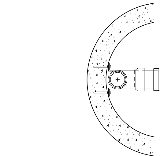
SECTION A-A CLAMP DETAIL
