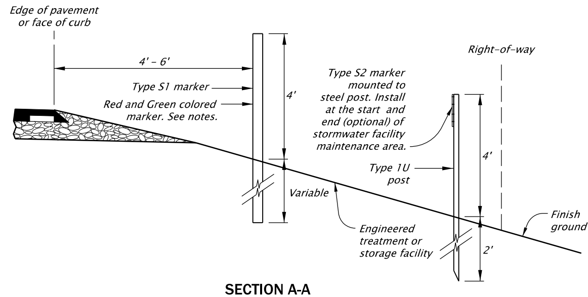
TYPE S1 & S2 MARKERS INSTALLATION DETAIL
