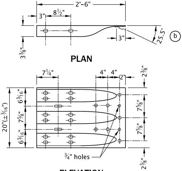
THRIE BEAM TERMINAL CONNECTOR
