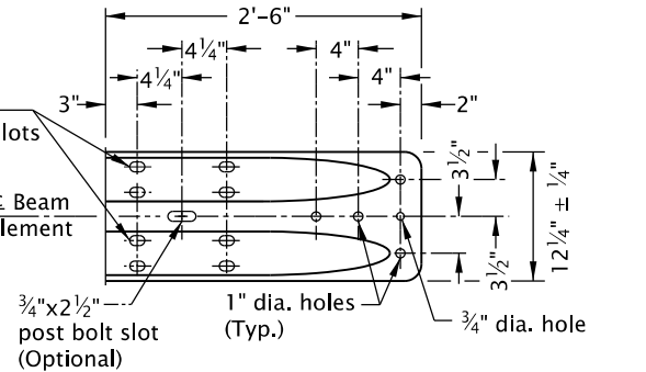
W-BEAM TERMINAL CONNECTOR
