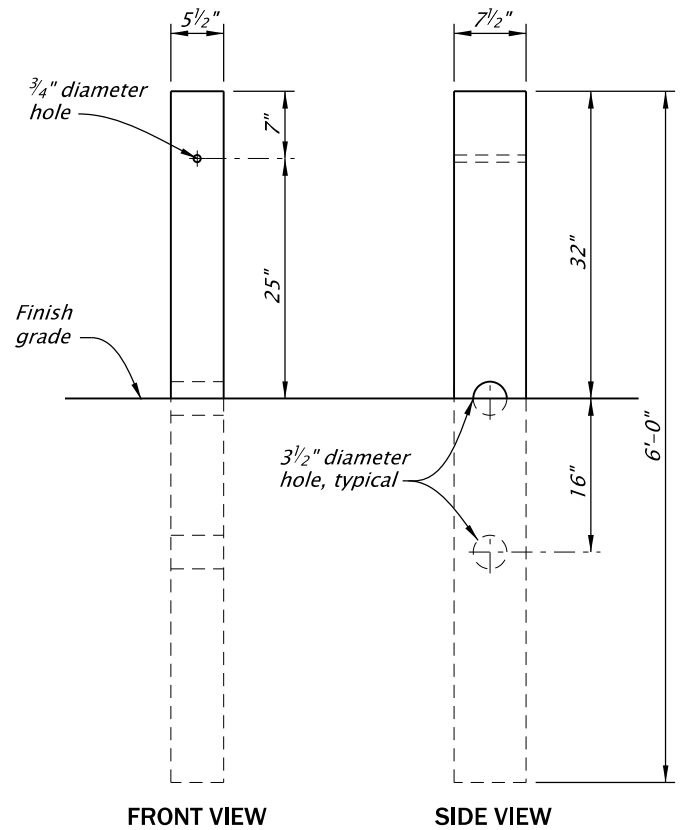
TOP OF RAIL HEIGHT 31" CONTROLLED RELEASE TERMINAL (CRT) POST
