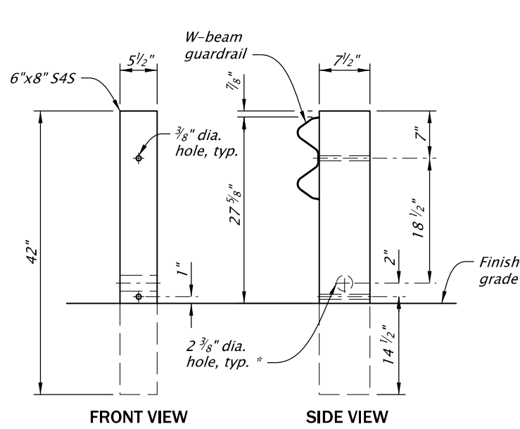
TOP OF RAIL HEIGHT 27 5 / 8 " This detail is retained for maintenance purposes only. Do not use for new construction.
