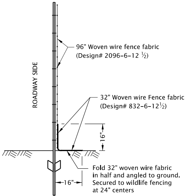
SECTION AT LINE POSTS
