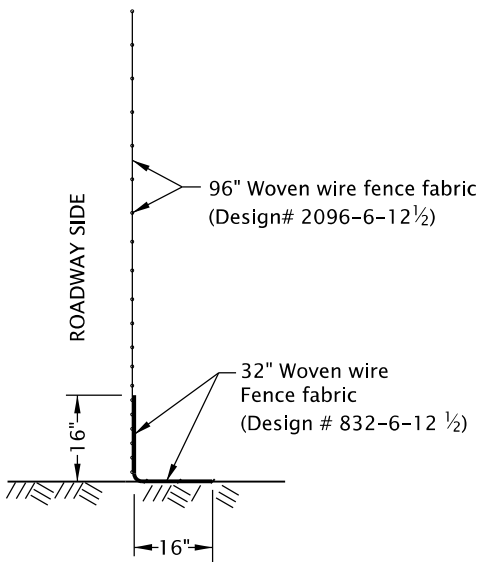
SECTION BETWEEN POSTS
