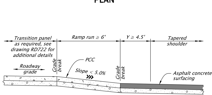
BLENDed TRANSITION TAPER OPTION "EW-3"
