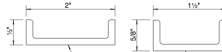
C" CHANNELS
