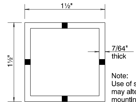
SQUARE TUBING
