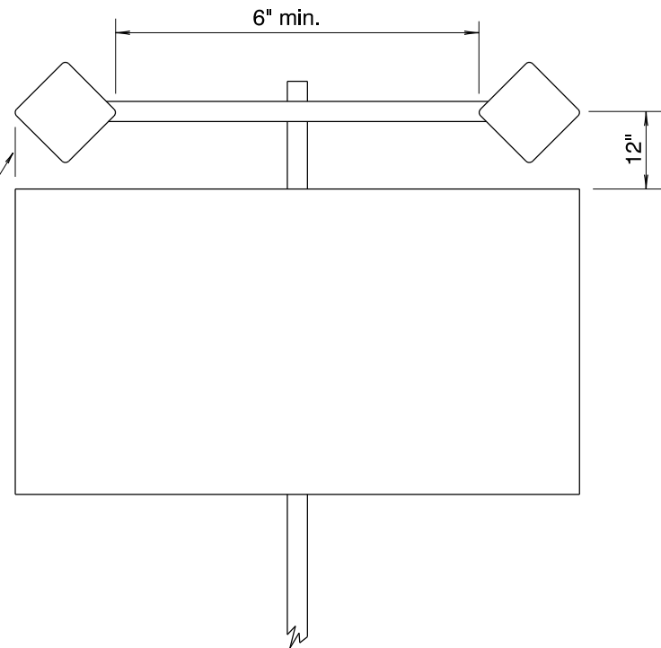
REGULATORY OR GUIDE SIGN (1 POST)
