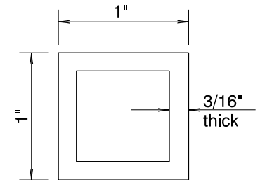
SQUARE TUBING
