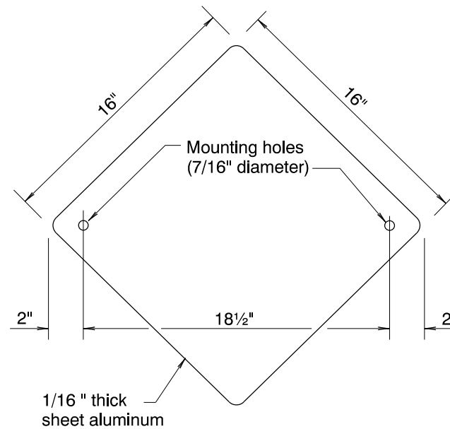
FLAG DETAILS
