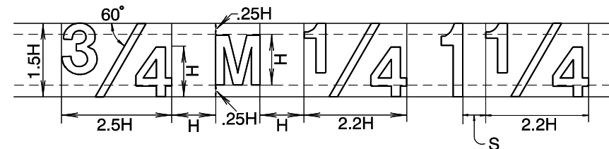
FRACTIONAL LAYOUT
