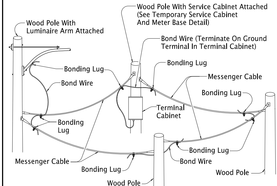
TEMPORARY GROUNDING/BONDING
