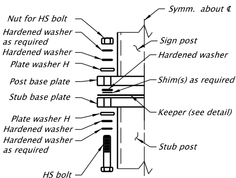
BASE ASSEMBLY DETAIL No Scale
