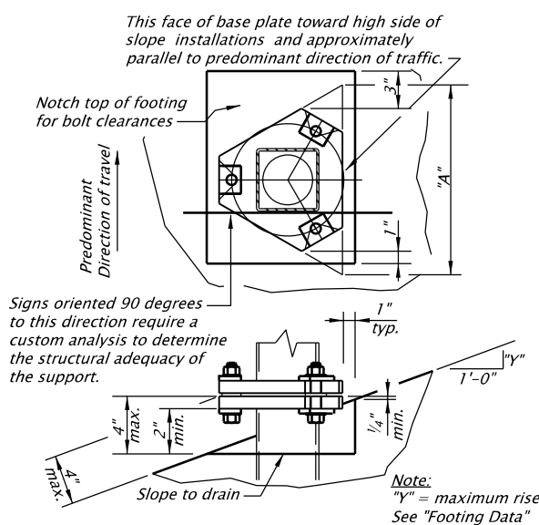
BASE PLATE ORIENTATION No Scale
