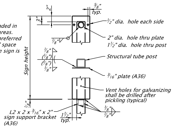
EXTRUDED SIGN MOUNTING DETAILS No Scale For signs 9'-0" or less in width
