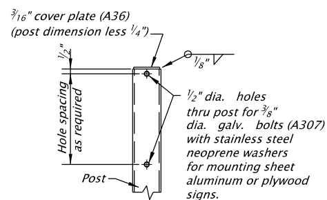
SIGN MOUNTING DETAILS FOR PLYWOOD & SHEET ALUMINUM SIGNS No Scale
