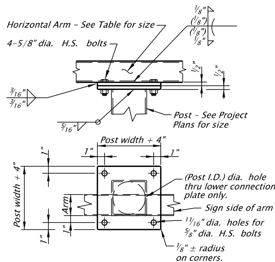
HORIZONTAL ARM TO POST CONNECTION DETAIL No Scale
