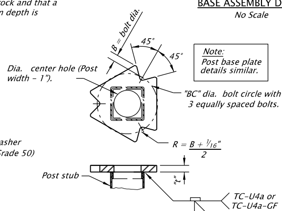
POST STUB DETAILS No Scale
