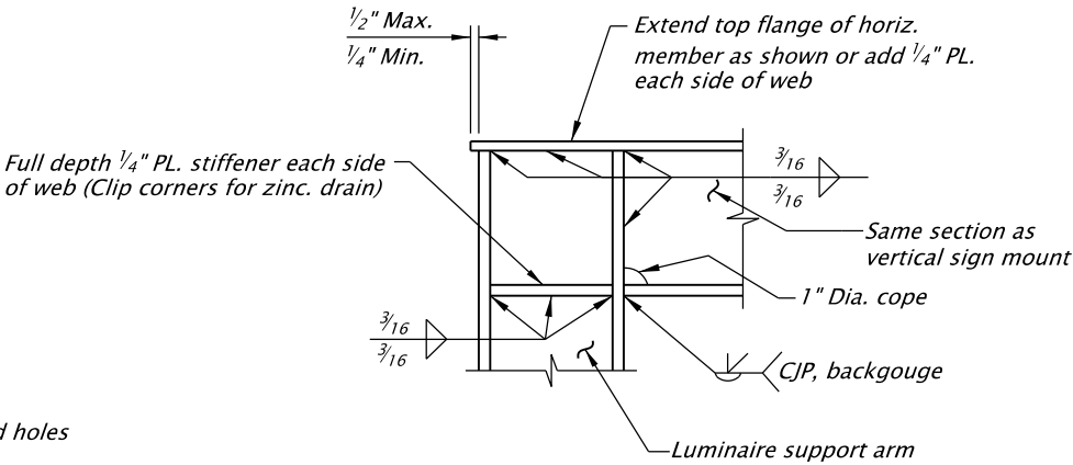
CORNER DETAIL No Scale
