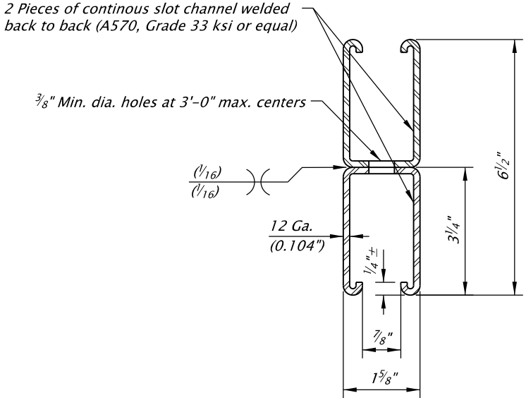
LUMINAIRE SUPPORT CHANNEL No Scale
