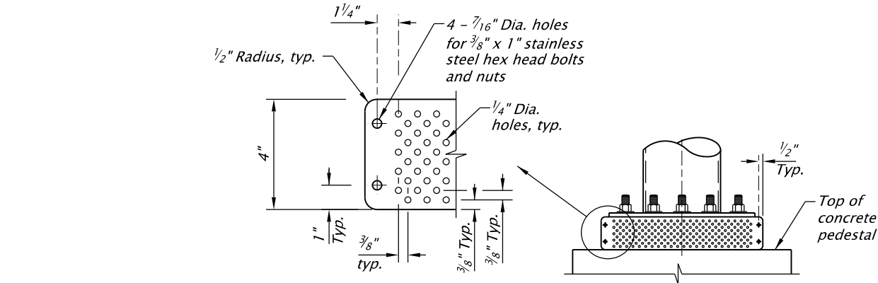
ELEVATION – RAT BAND No Scale
