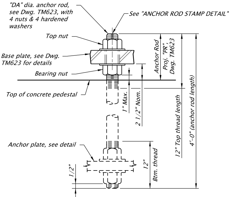
DETAILS @ TOP AND BOTTOM OF ANCHOR ROD No Scale
