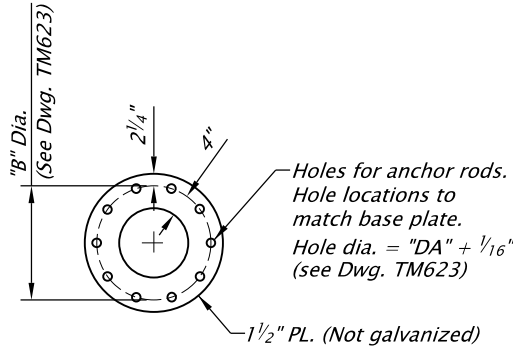
ANCHOR PLATE DETAIL No Scale
