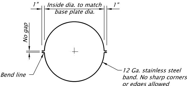
PLAN – RAT BAND No Scale
