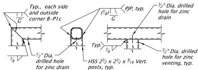
SAFETY RAIL – WELD DETAILS
