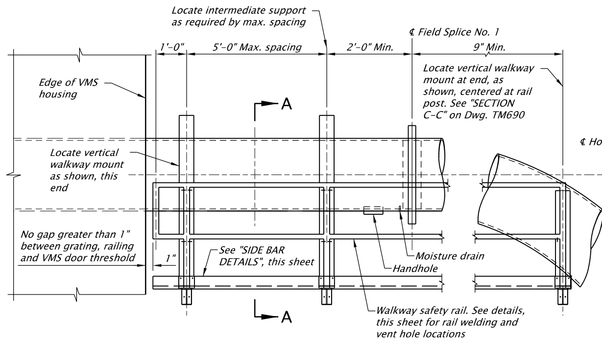
WALKWAY EXTENSION DETAILS
