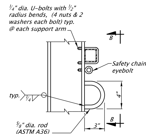
DETAIL "C" No Scale
