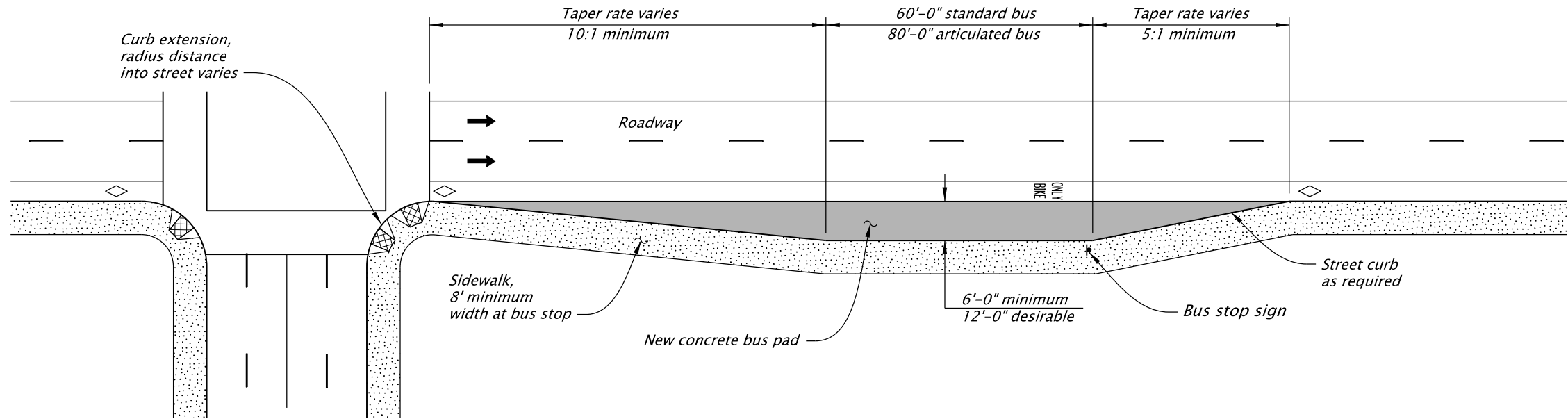
BUS TURNOUT WITH BIKE LANE
