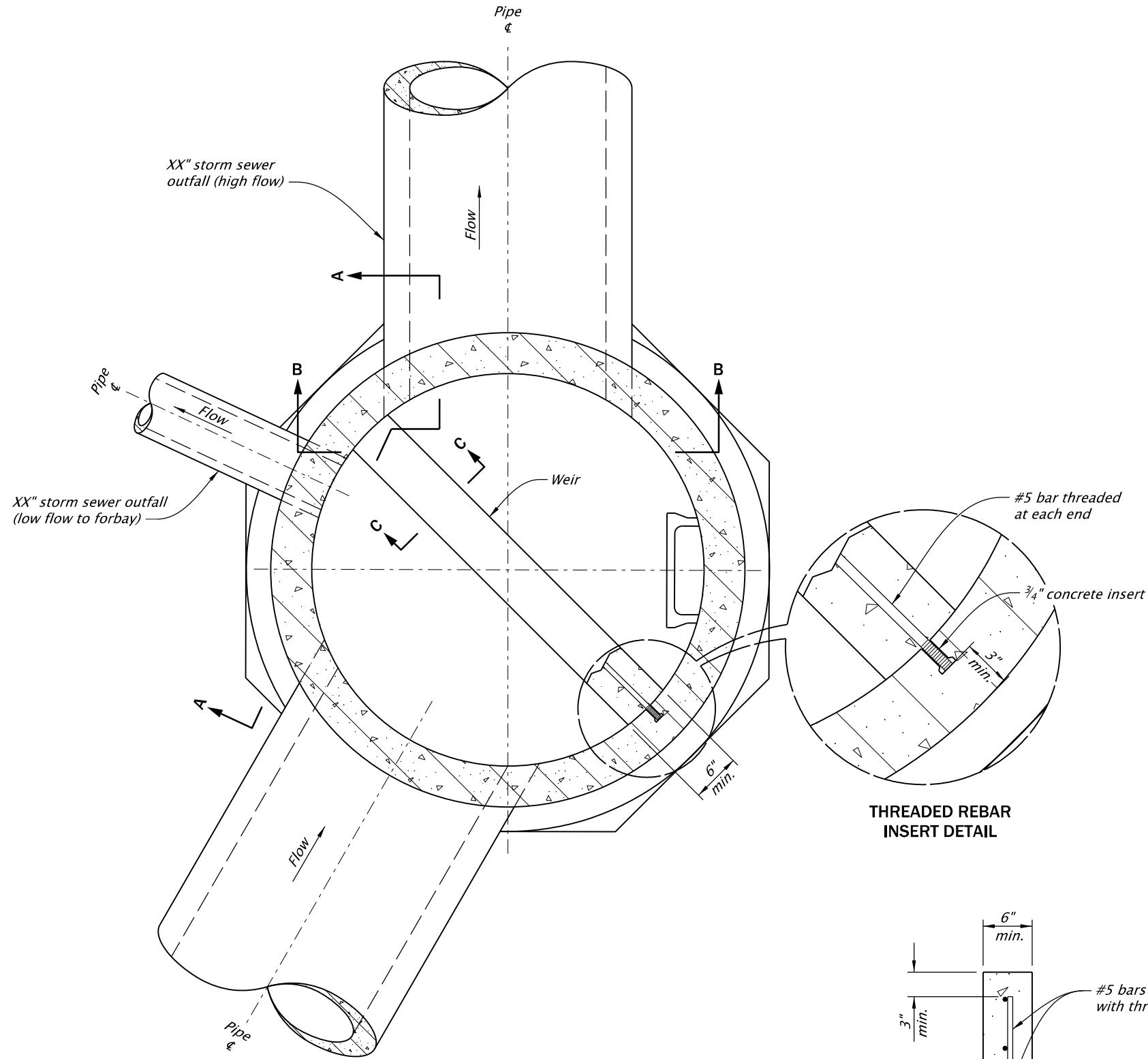
XX" MANHOLE PLAN
