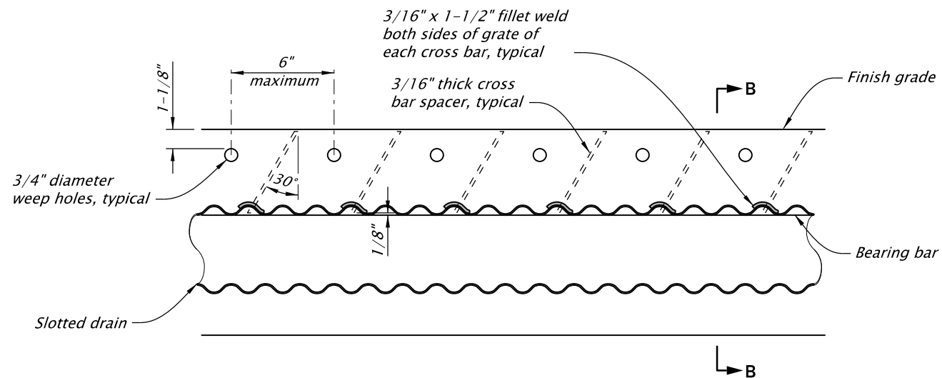
WEEP HOLES DETAIL
