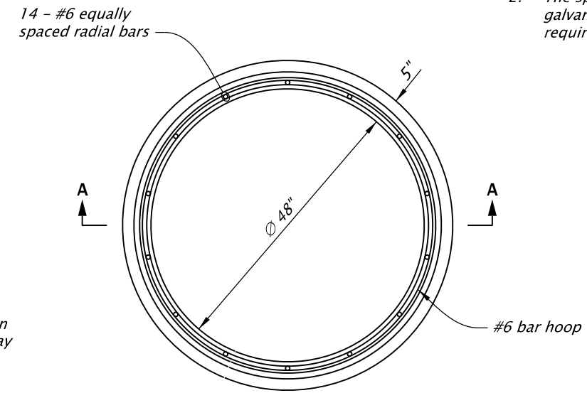
RISER PLAN AT TOP OF RIM
