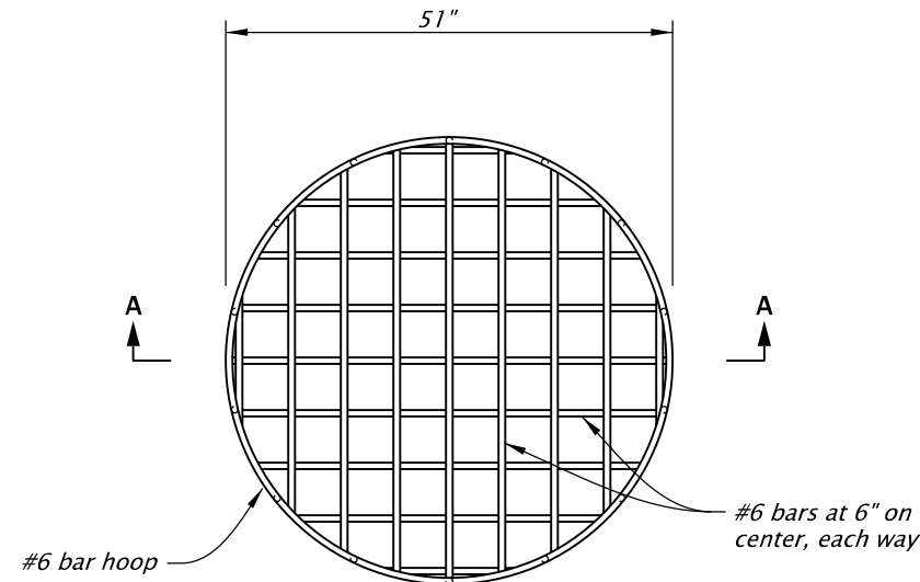
RISER COVER PLAN
