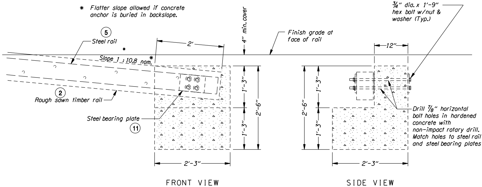
CONCRETE ANCHOR
