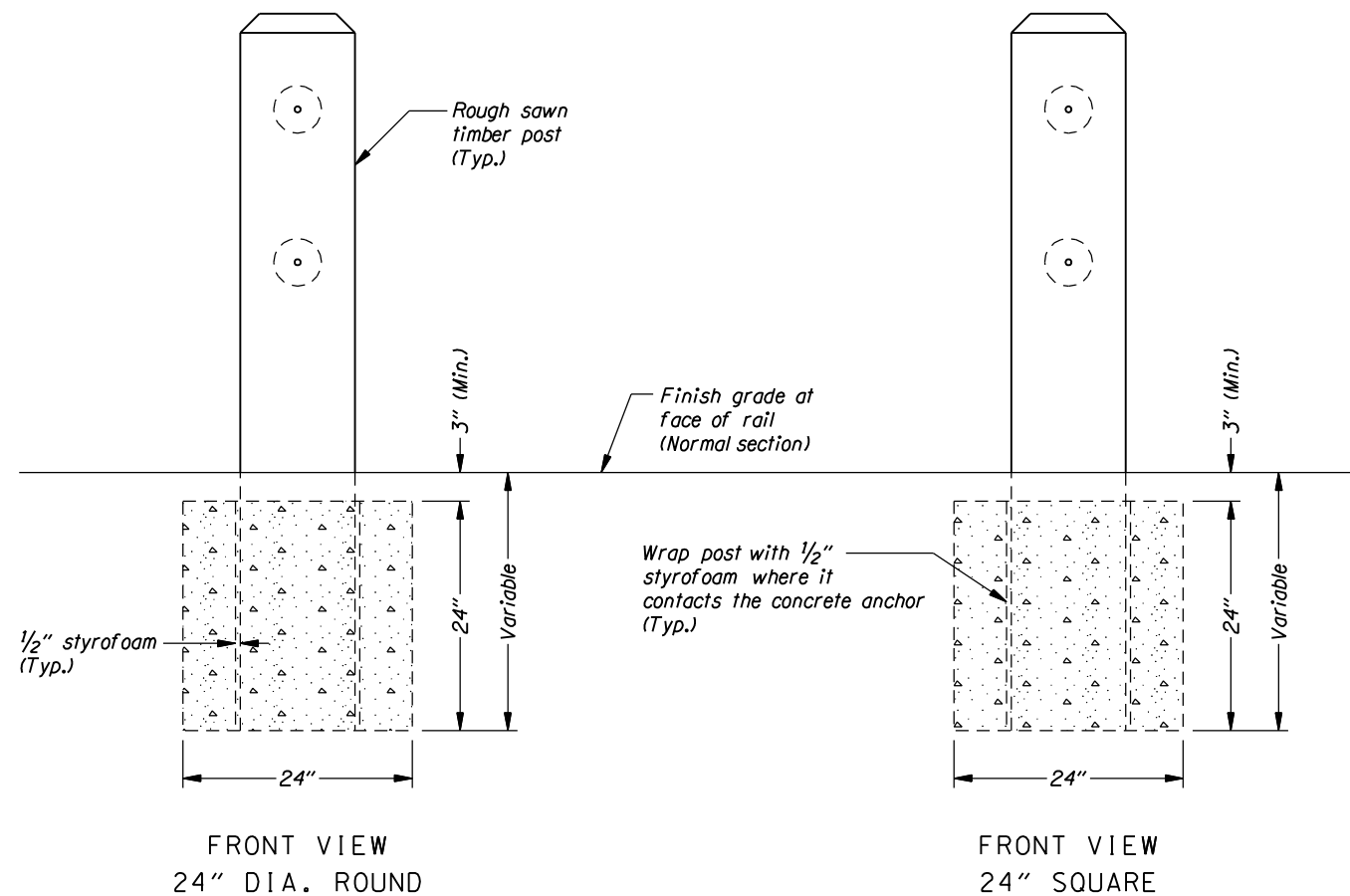
CONCRETE ANCHORS FOR SHORT GUARDRAIL POST (Reduced size acceptable in solid rock)
