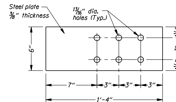
STEEL TERMINAL SECTION (35)
