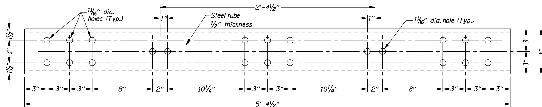
HSS (STEEL TUBE) 6" x 4" x 1/2" (30)
