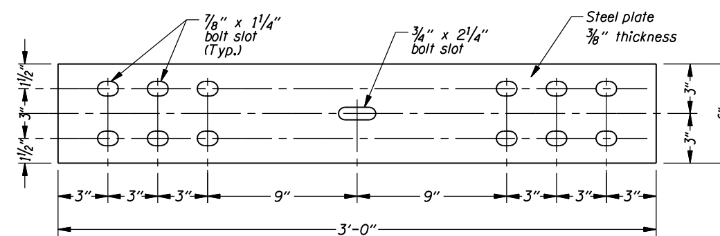
STEEL SPLICE PLATE (33)
