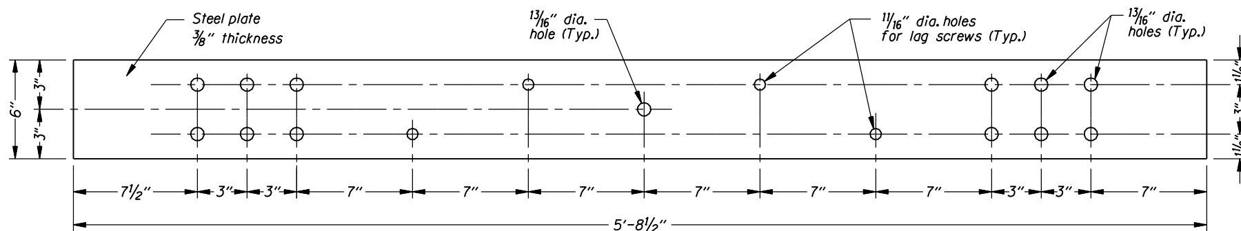
STEEL TERMINAL SECTION (32)
