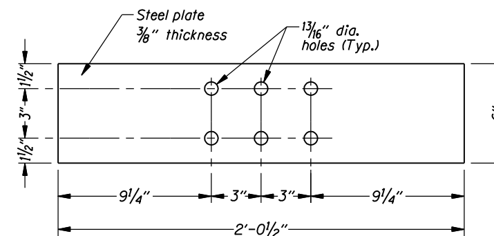
STEEL TERMINAL SECTION (34)
