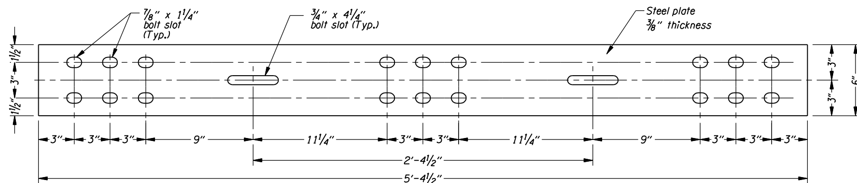
STEEL SPLICE PLATE (31)
